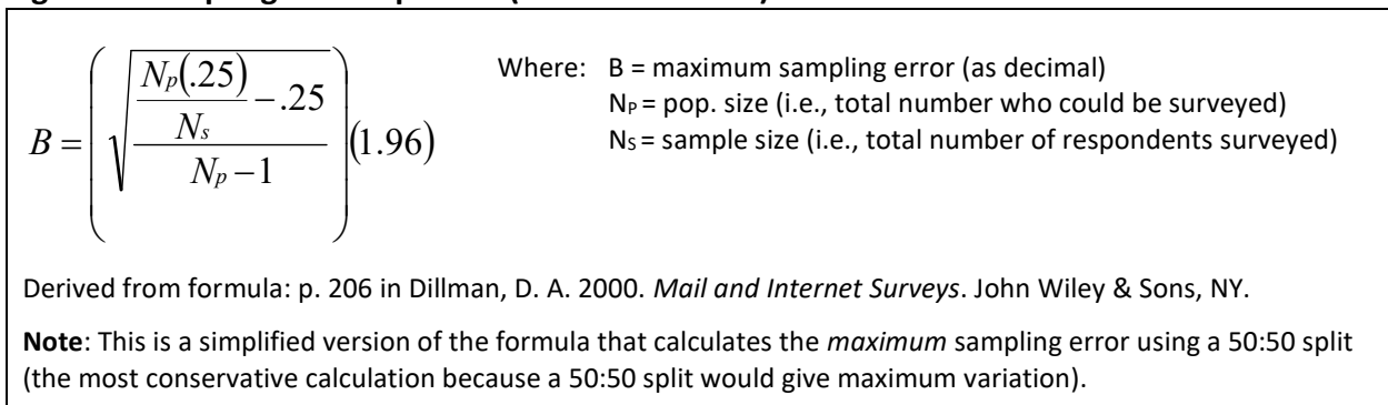
Figure 3. Sampling Error Equation (Dillman Method)
