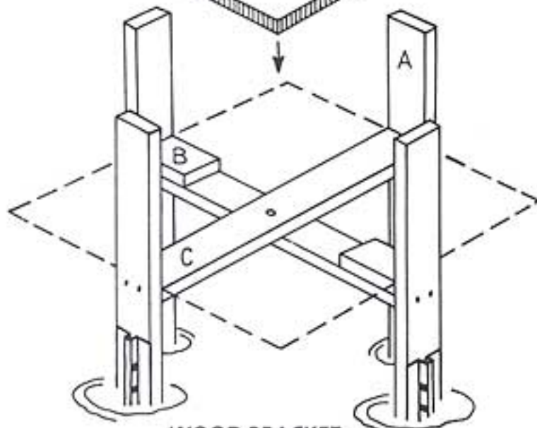
WOOD BRACKET
