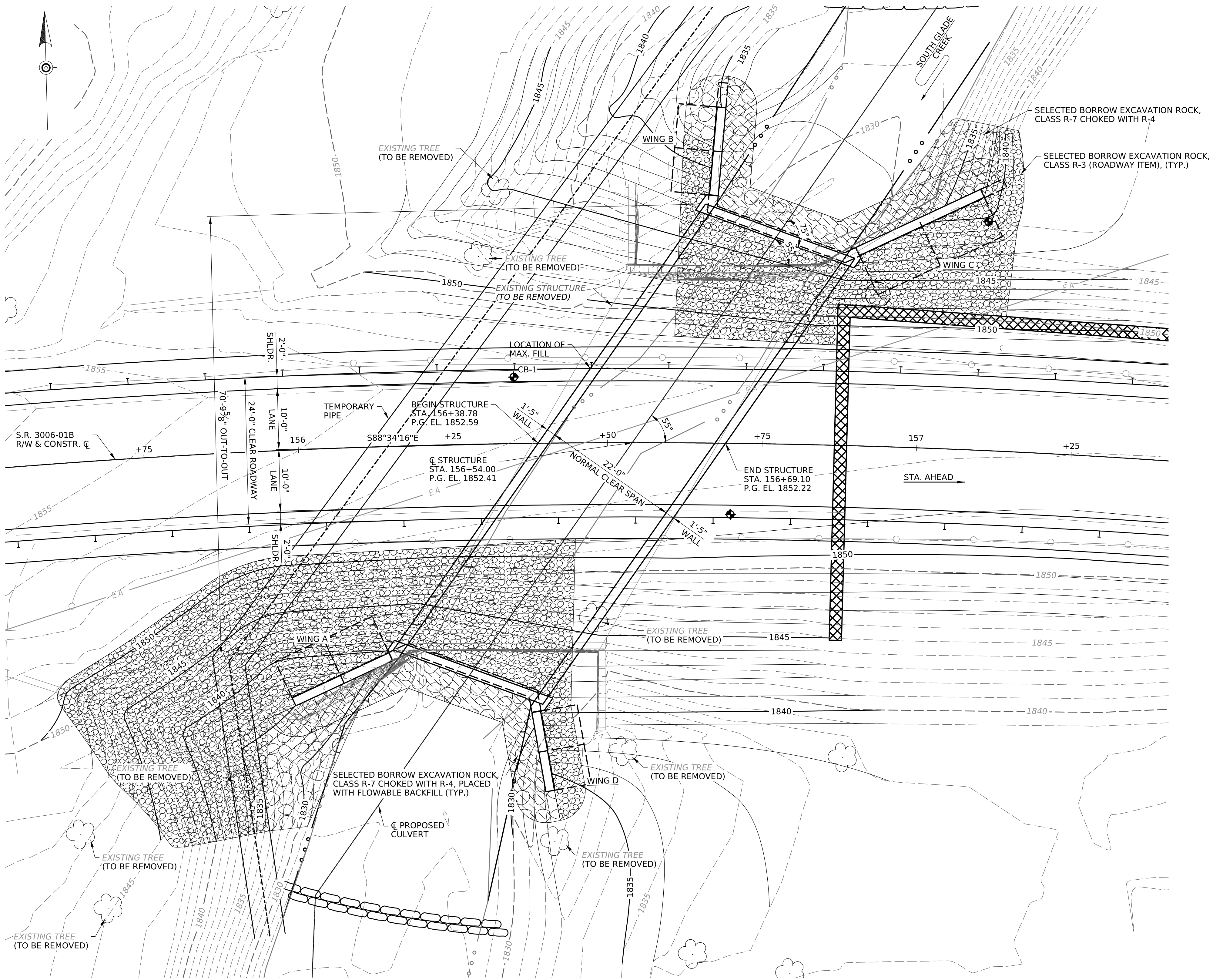
PLAN VIEW
