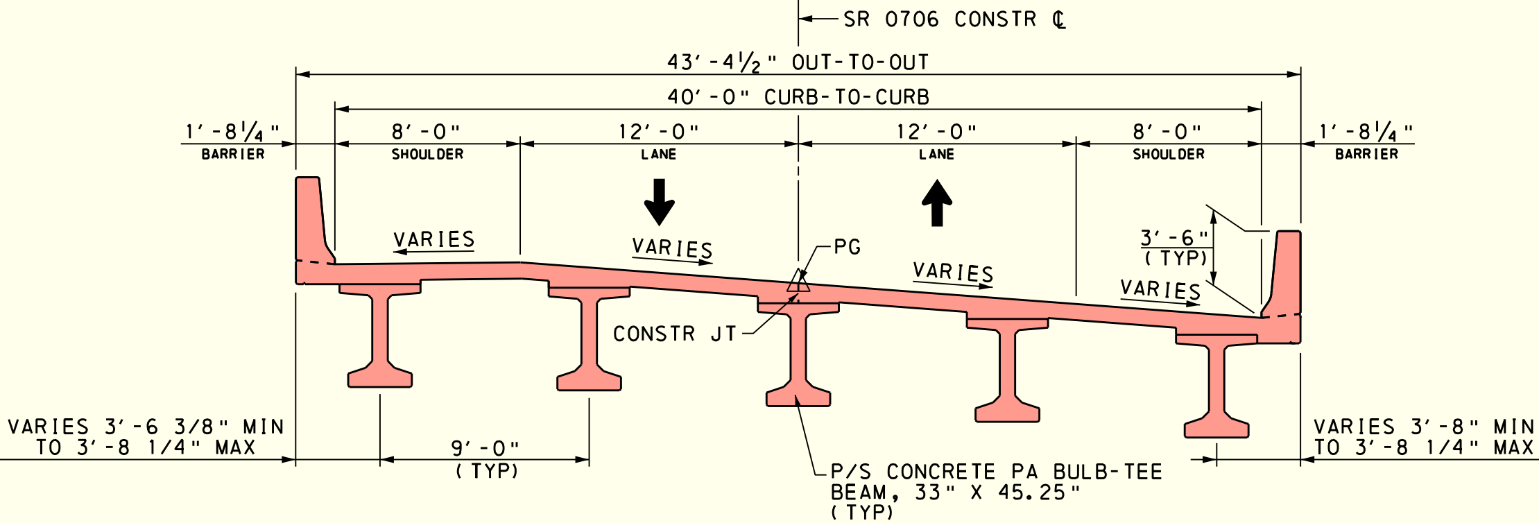
PROPOSED BRIDGE TYPICAL SECTION
