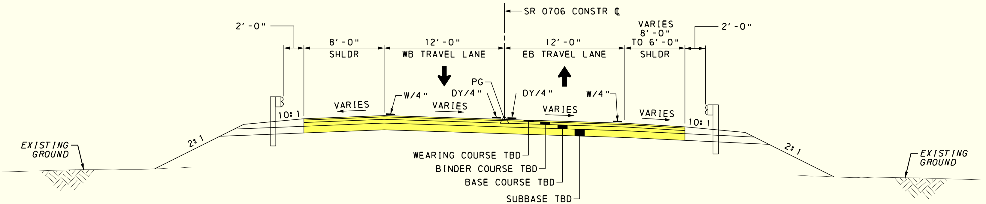
SR 0706 - TYPICAL ROADWAY SECTION
