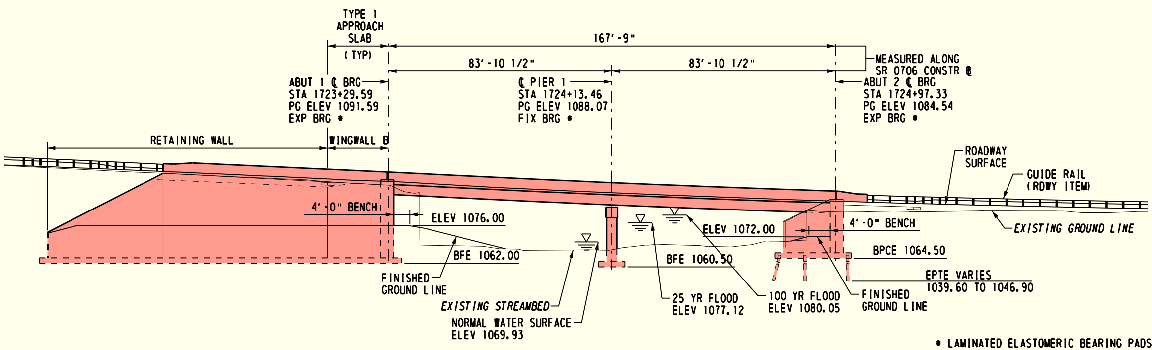
PROPOSED BRIDGE ELEVATION VIEW
