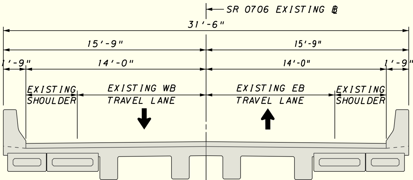
EXISTING BRIDGE TYPICAL SECTION
