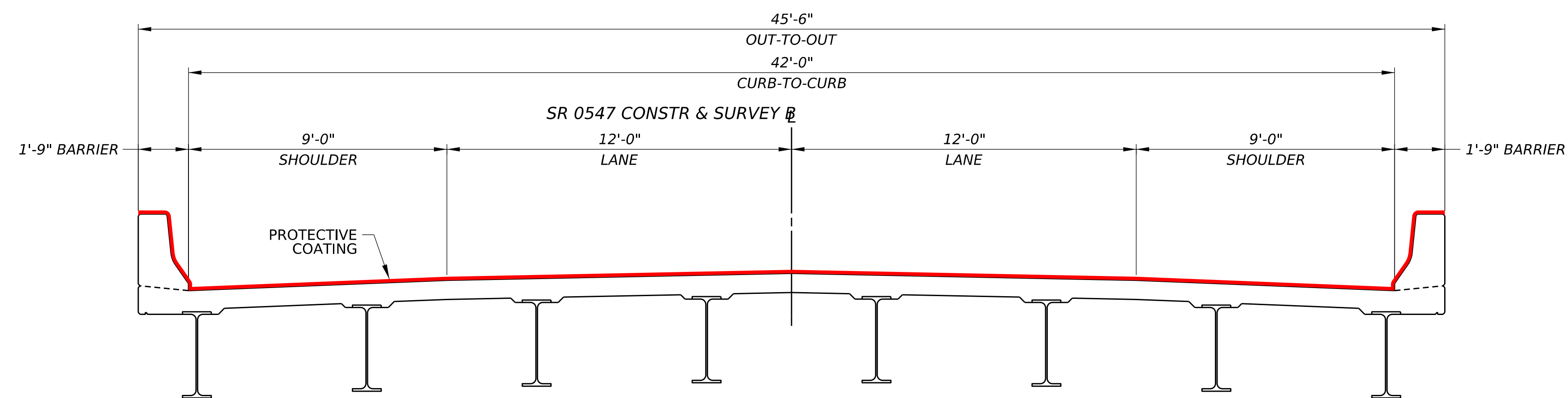
PROPOSED TYPICAL SECTION
