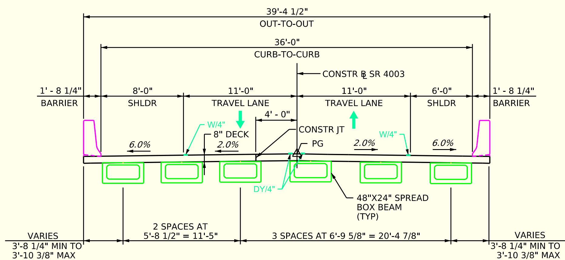
PROPOSED BRIDGE TYPICAL SECTION
