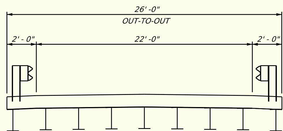
EXISTING BRIDGE TYPICAL SECTION
