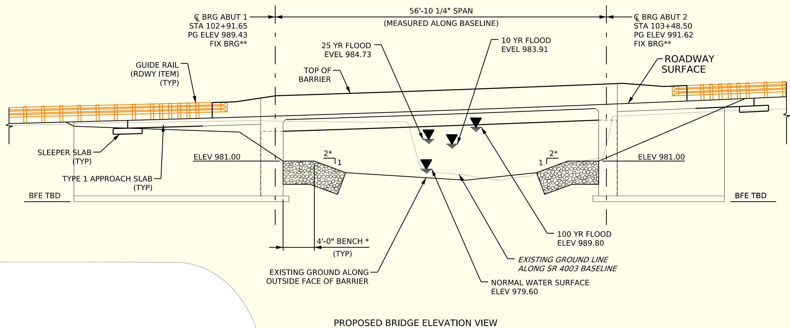
PROPOSED BRIDGE ELEVATION VIEW
