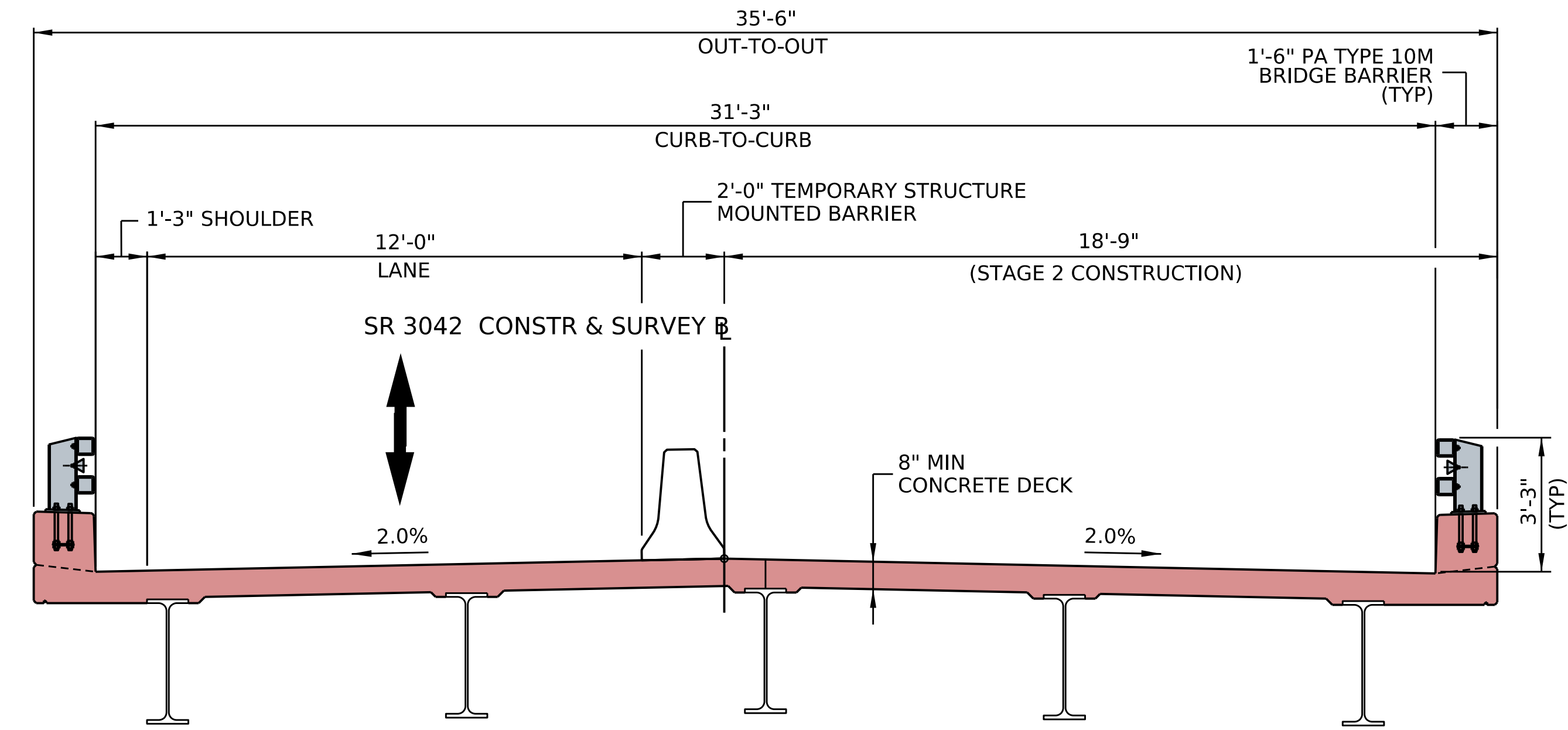
STAGE 2 TYPICAL SECTION
