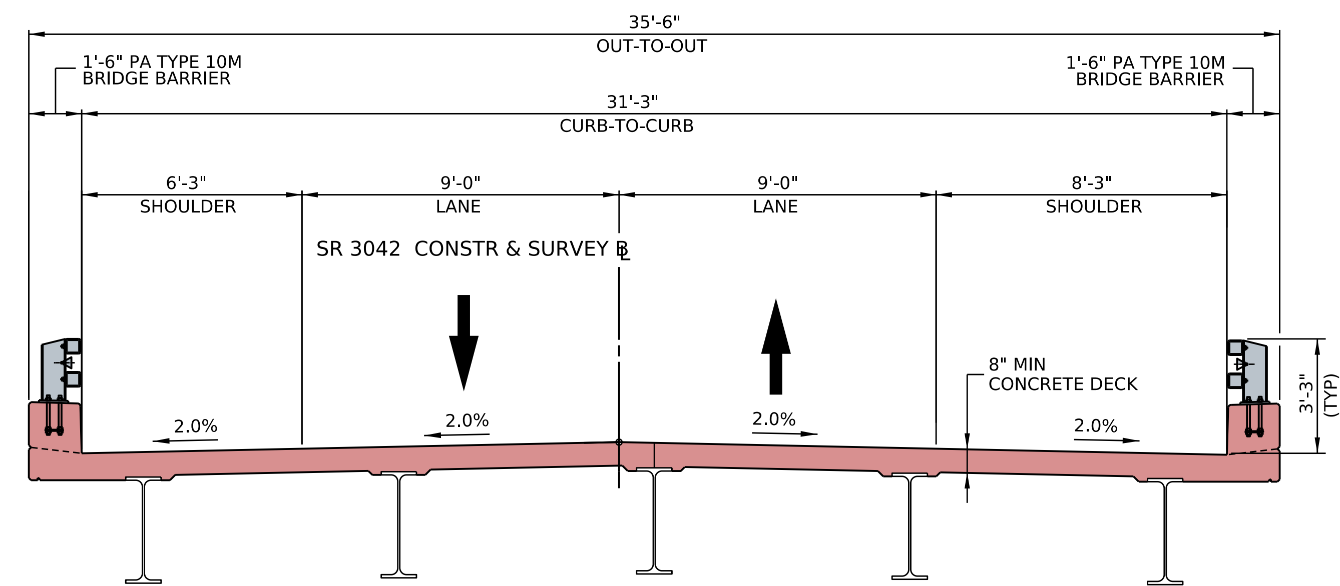
PROPOSAL TYPICAL SECTION
