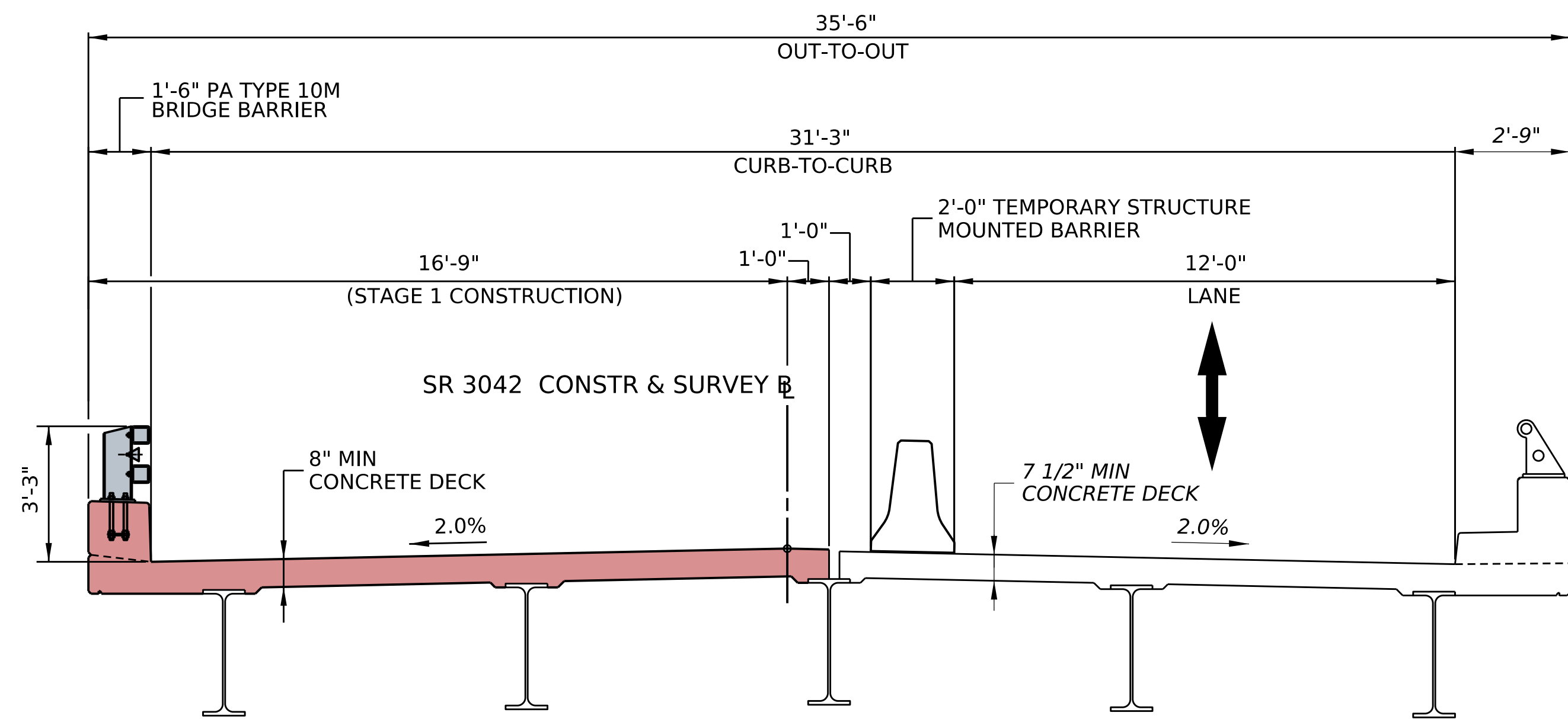
STAGE 1 TYPICAL SECTION
