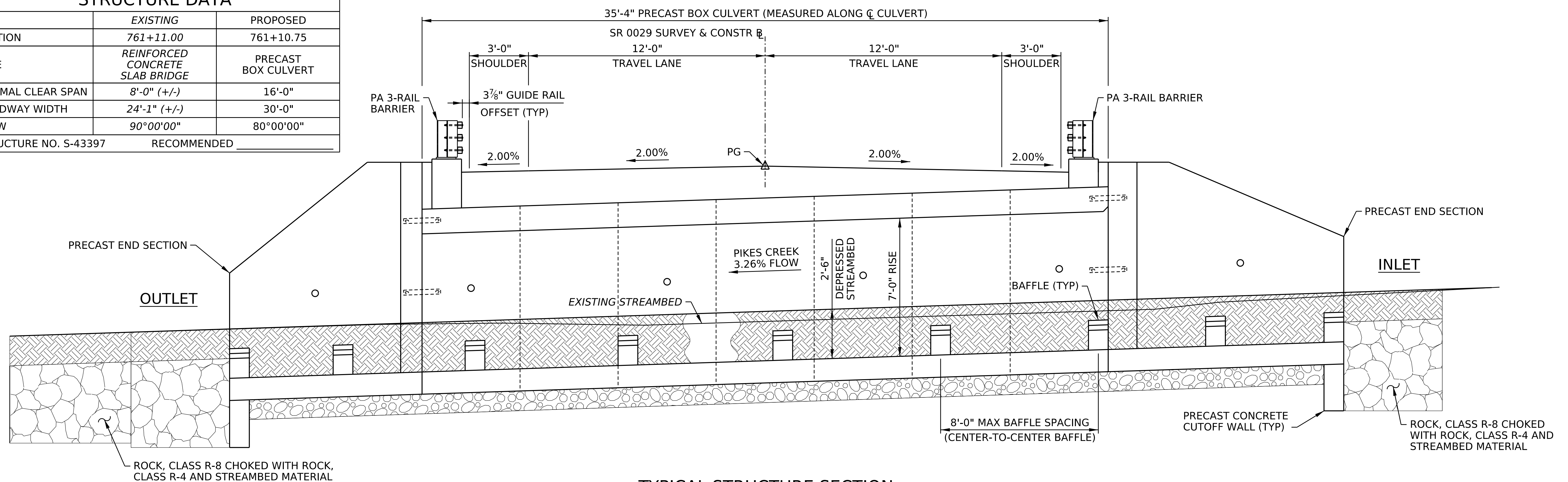
TYPICAL STRUCTURE SECTION NOT TO SCALE
