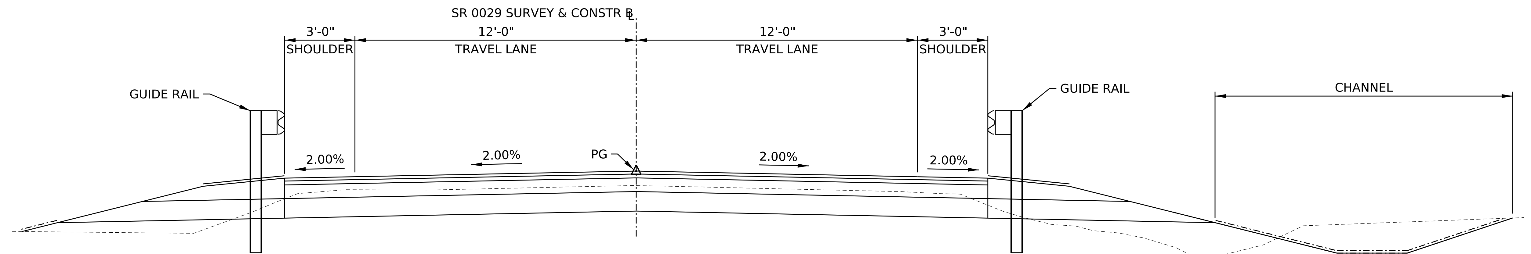
TYPICAL ROADWAY SECTION NOT TO SCALE
