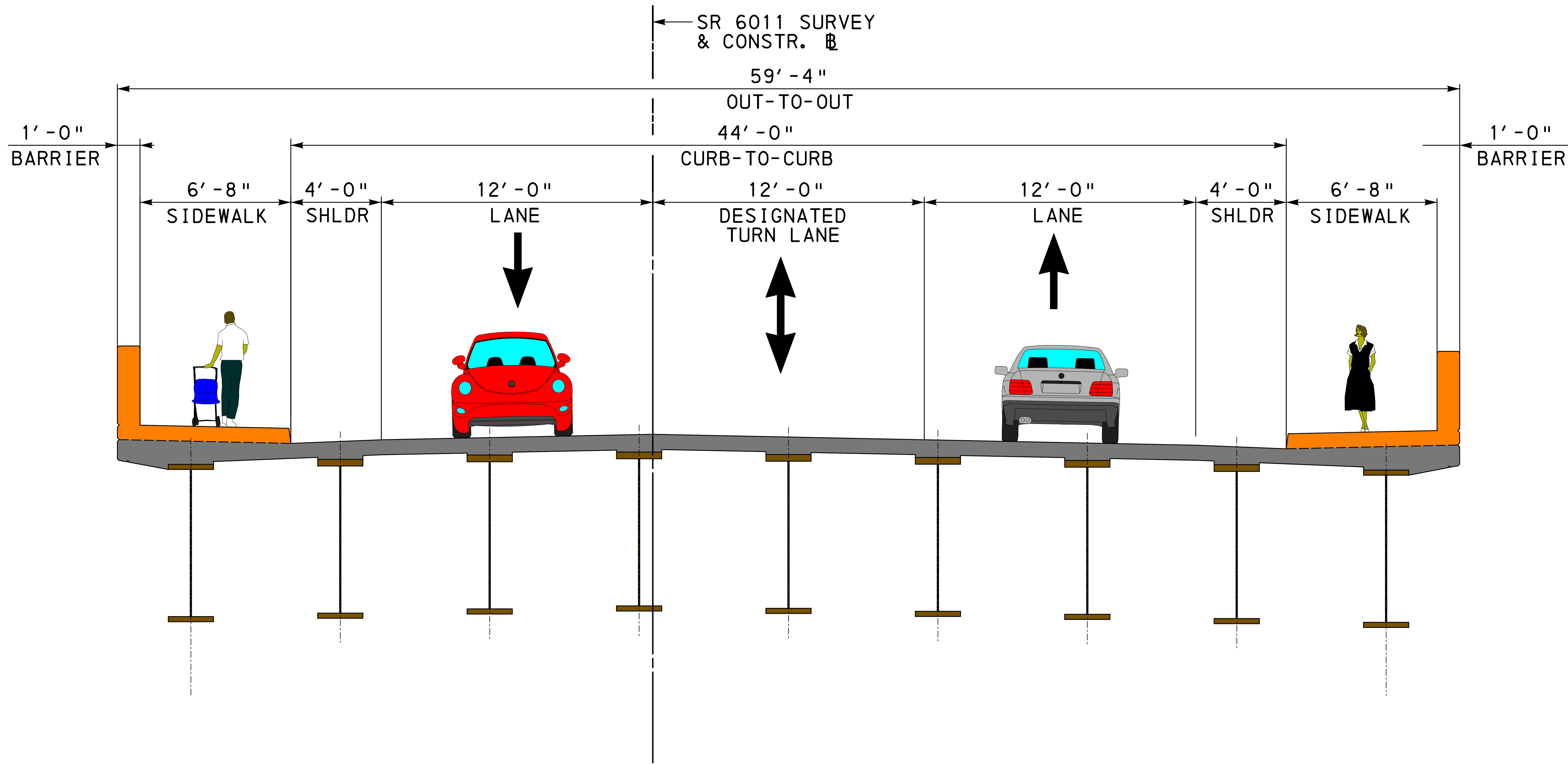
PROPOSED STRUCTURE - TYPICAL SECTION NOT TO SCALE
