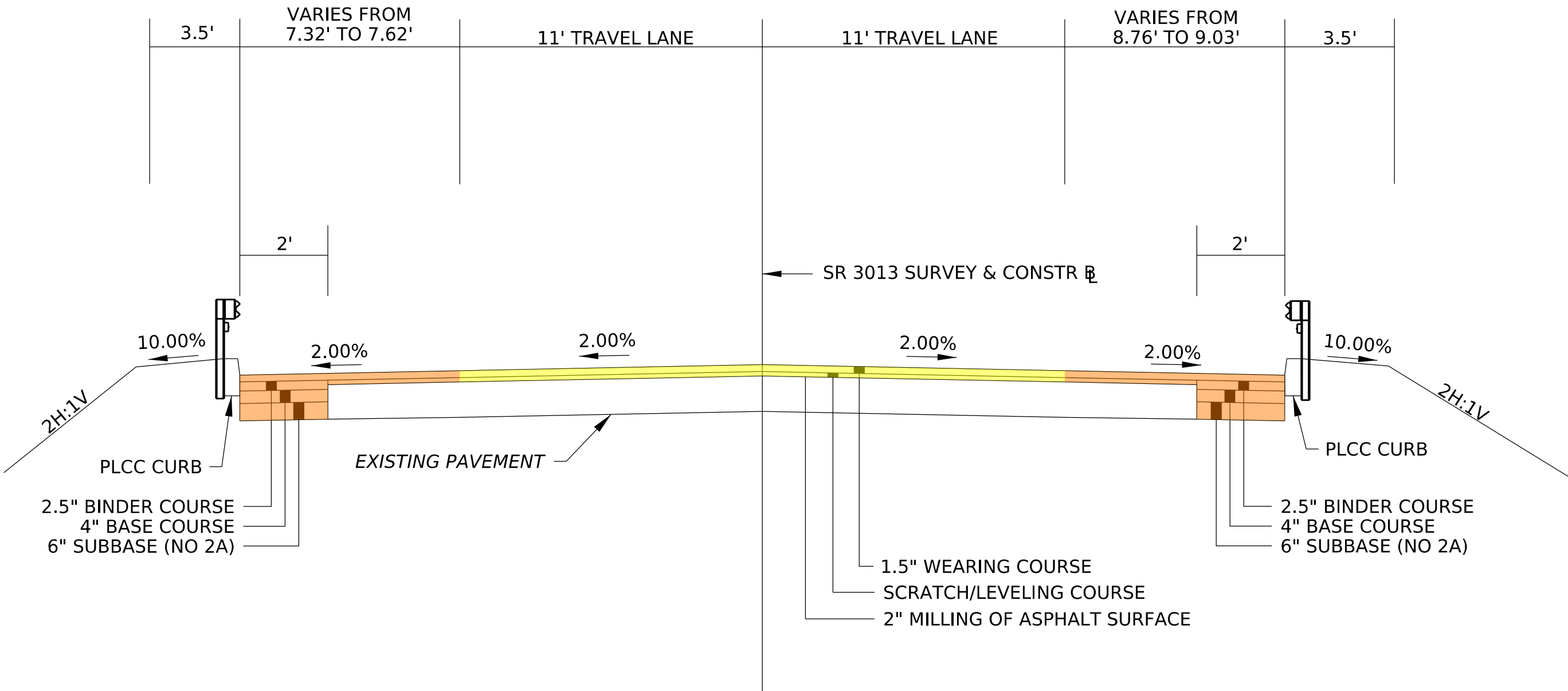
SR 3013 TYPICAL SECTION NOT TO SCALE
