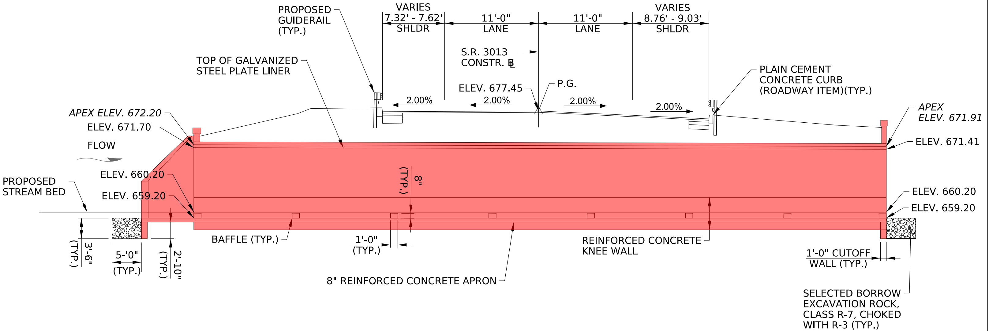
SR 3013 BRIDGE REHABILITATION SECTION NOT TO SCALE
