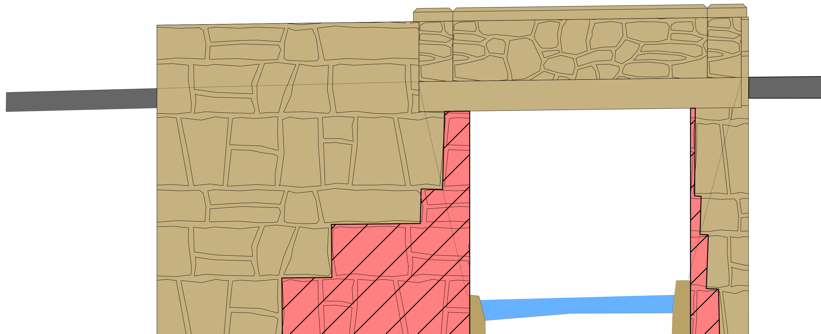
ELEVATION VIEW
