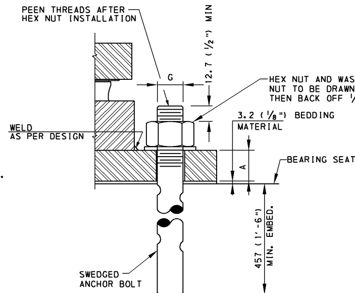
ALTERNATE POT PLATE ATTACHMENT
