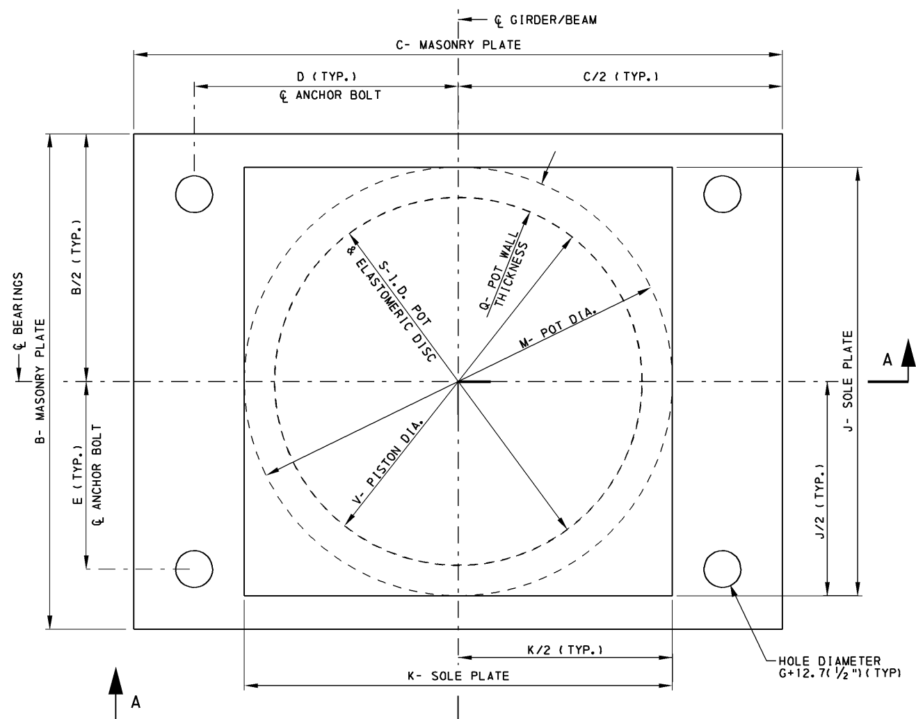
FIXED POT BEARING PLAN
