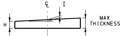
BEVELED SOLE PLATE DETAIL
