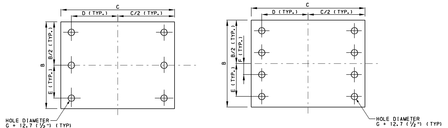
ANCHOR BOLT LOCATION PLAN - 6 AND 8 ANCHOR BOLTS
