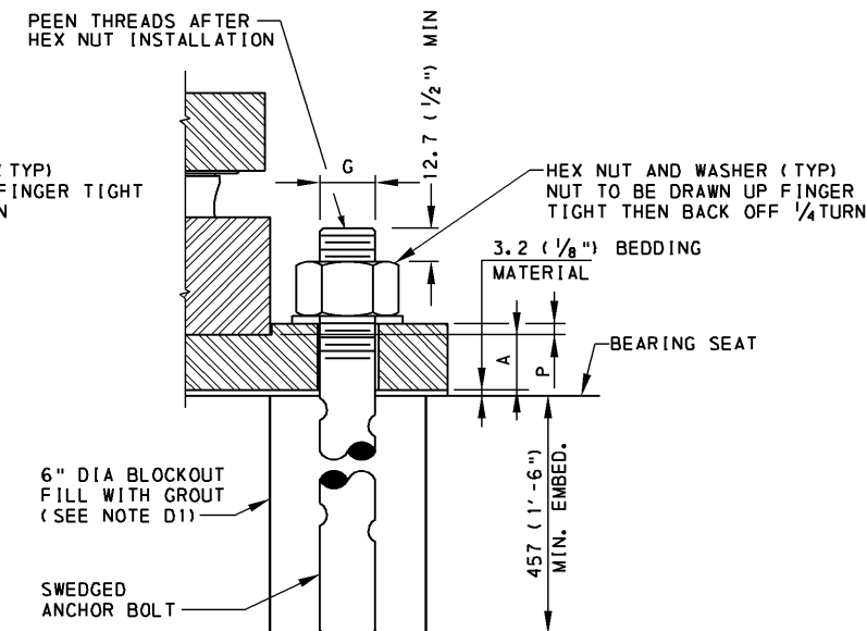
ANCHOR BOLT DETAIL 1
