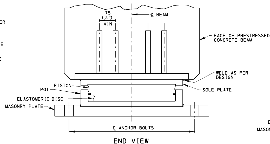
ANCHOR CONNECTION FOR PRESTRESSED CONCRETE BEAM
