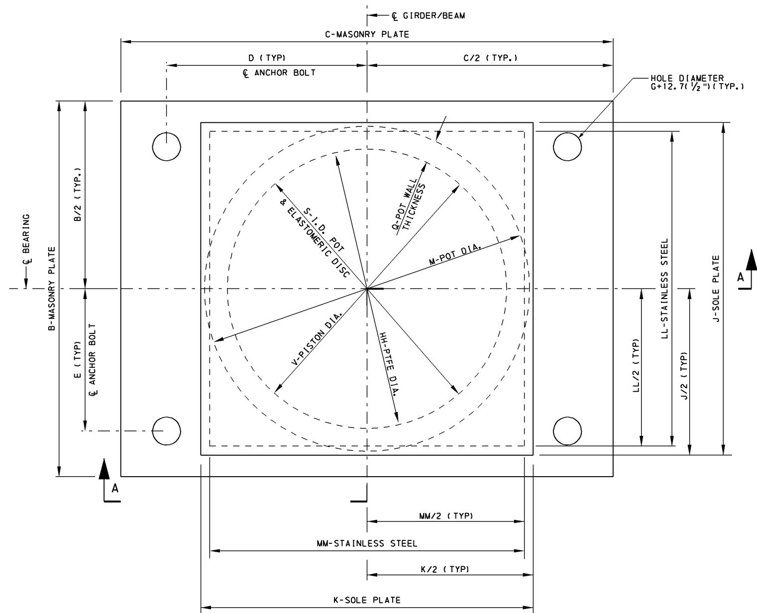
NON-GUIDED POT BEARING PLAN
