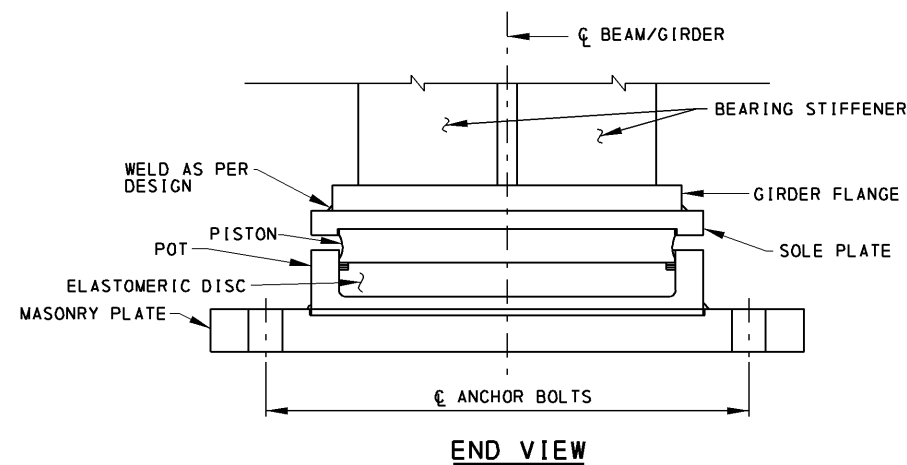
WELDED CONNECTION FOR STEEL BEAM
