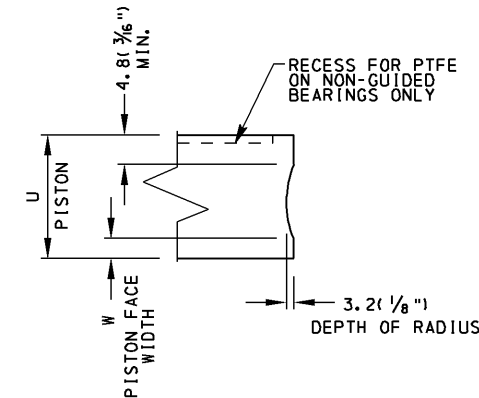
PISTON DETAIL
