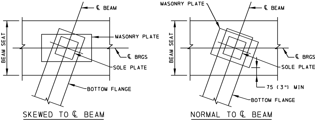
SOLE AND MASONRY PLATE ORIENTATION OPTIONS
