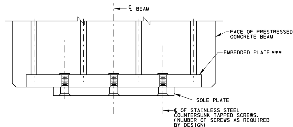
ALTERNATE TAPPED BOLT CONNECTION
