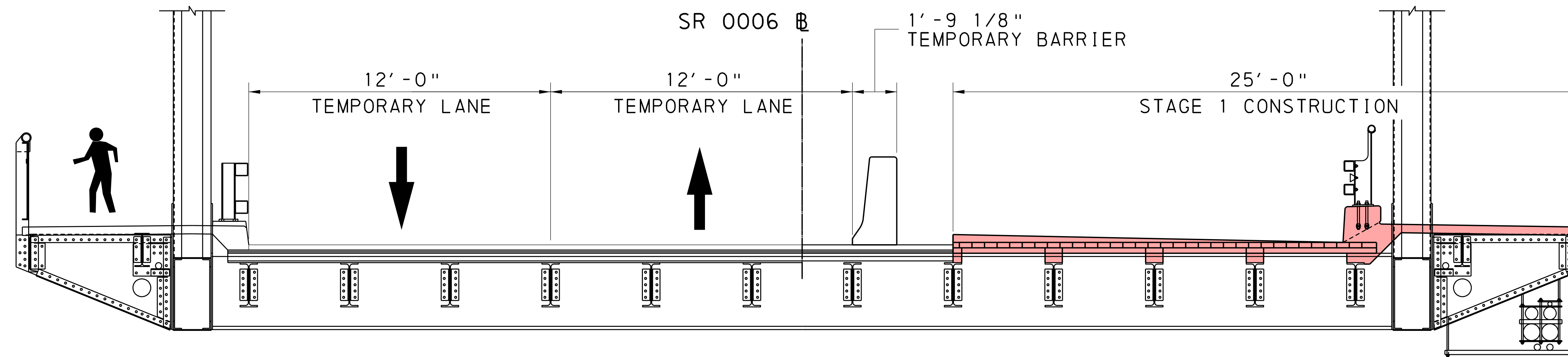
STAGE 1 TYPICAL SECTION
