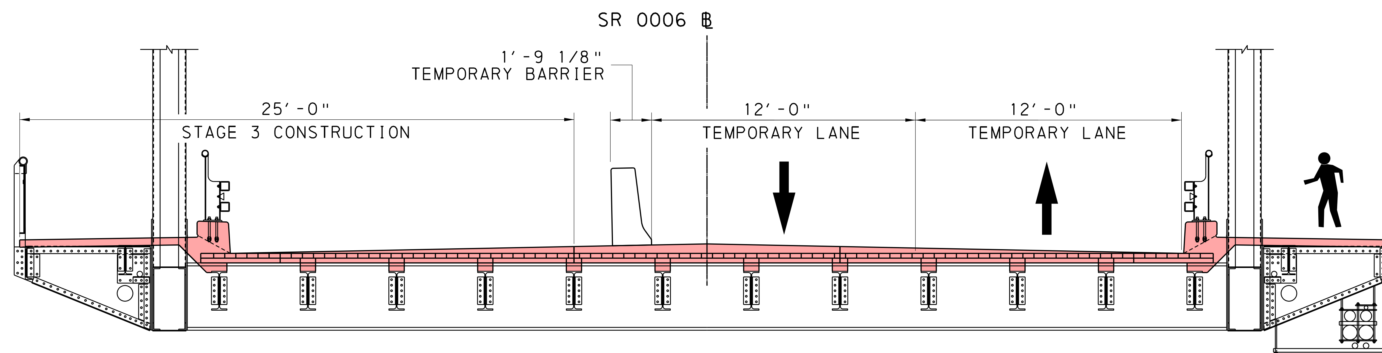
STAGE 3 TYPICAL SECTION
