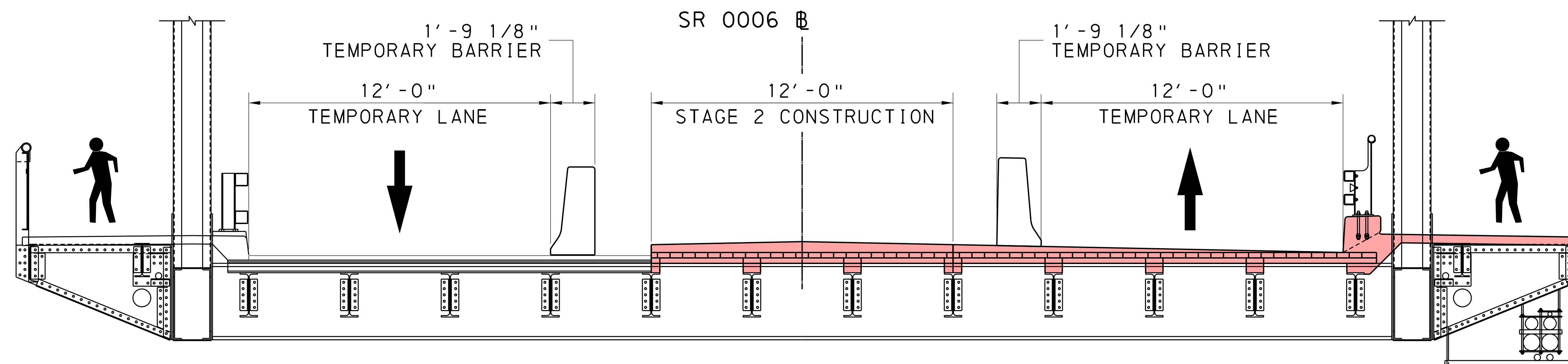
STAGE 2 TYPICAL SECTION
