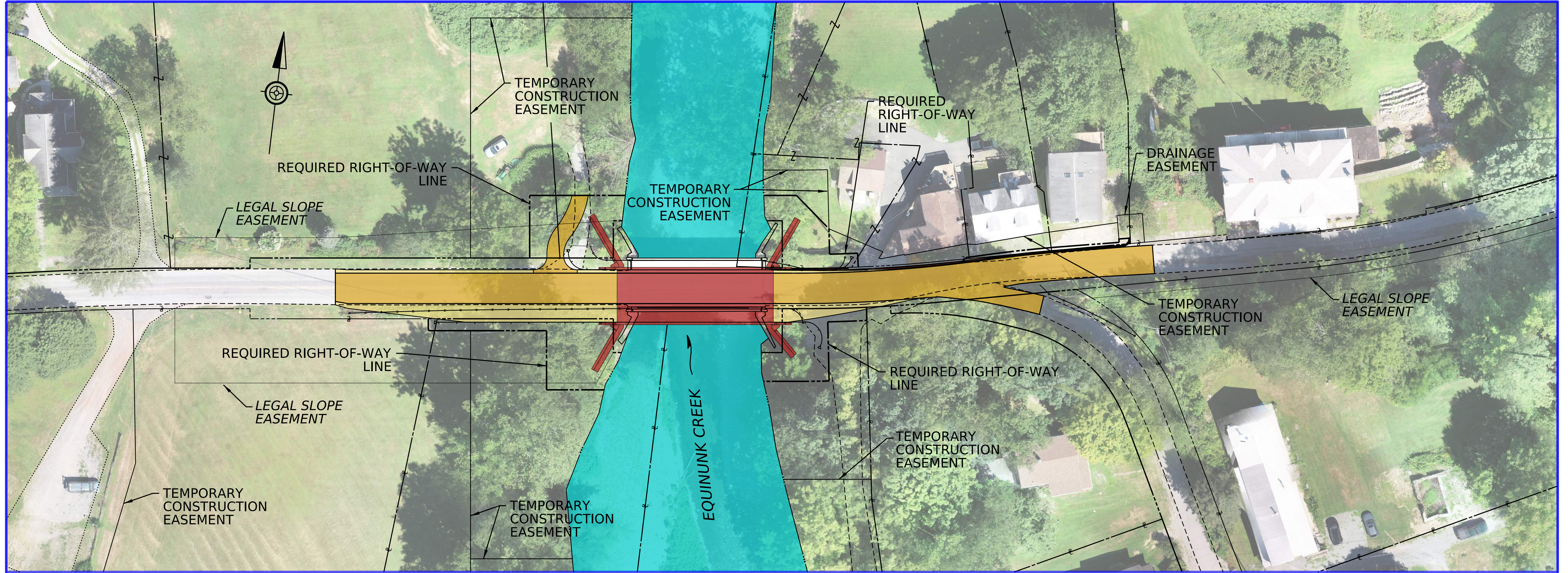
PLAN
