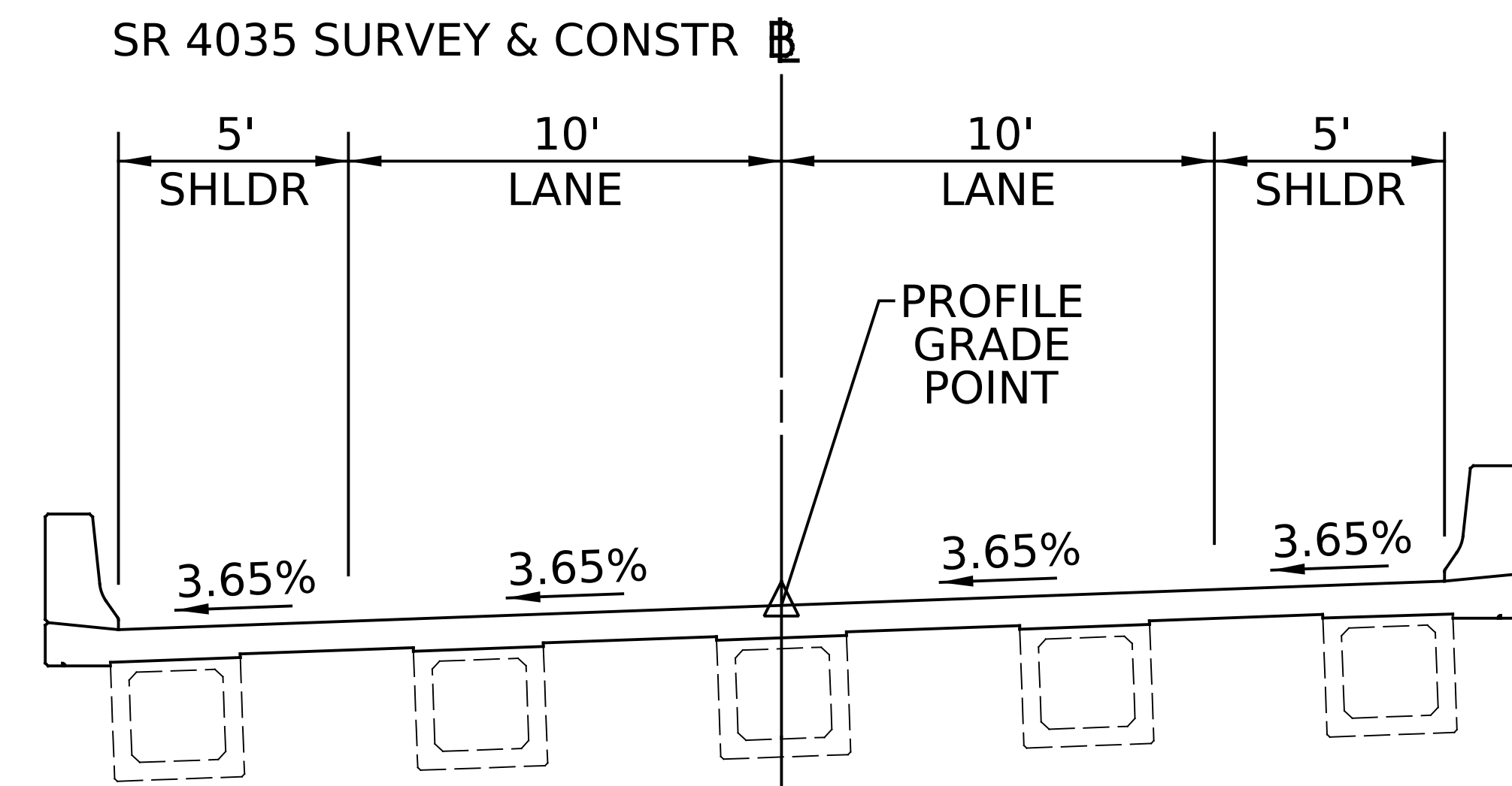
SR 4035 NORMAL SECTION (STRUCTURE)
