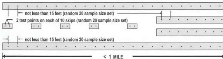
FIGURE 1 - TYPICAL TEST POINT LOCATION FOR ZONE OF MEASUREMENT LESS THAN 1 MILE
