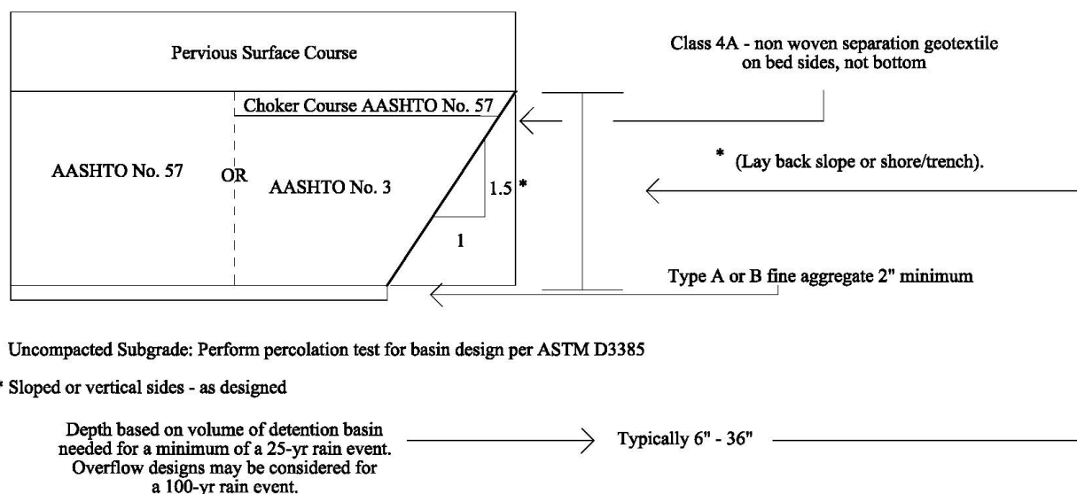
FIGURE K.1 PERVIOUS SYSTEM DESIGN
