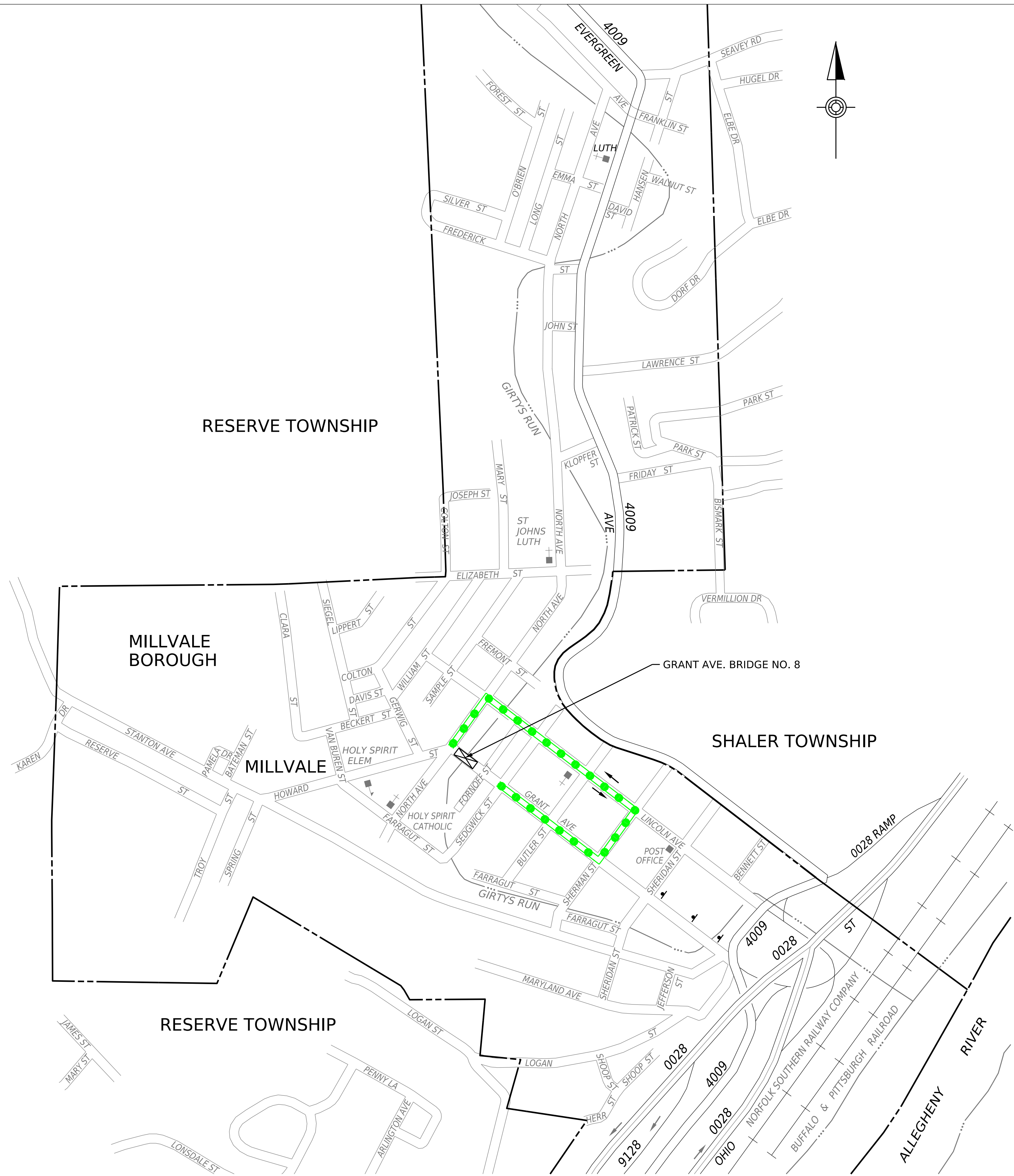
GRANT AVENUE BRIDGE NO. 8 DETOUR PLAN DETOUR LENGTH = 0.3 MILES NOT TO SCALE
