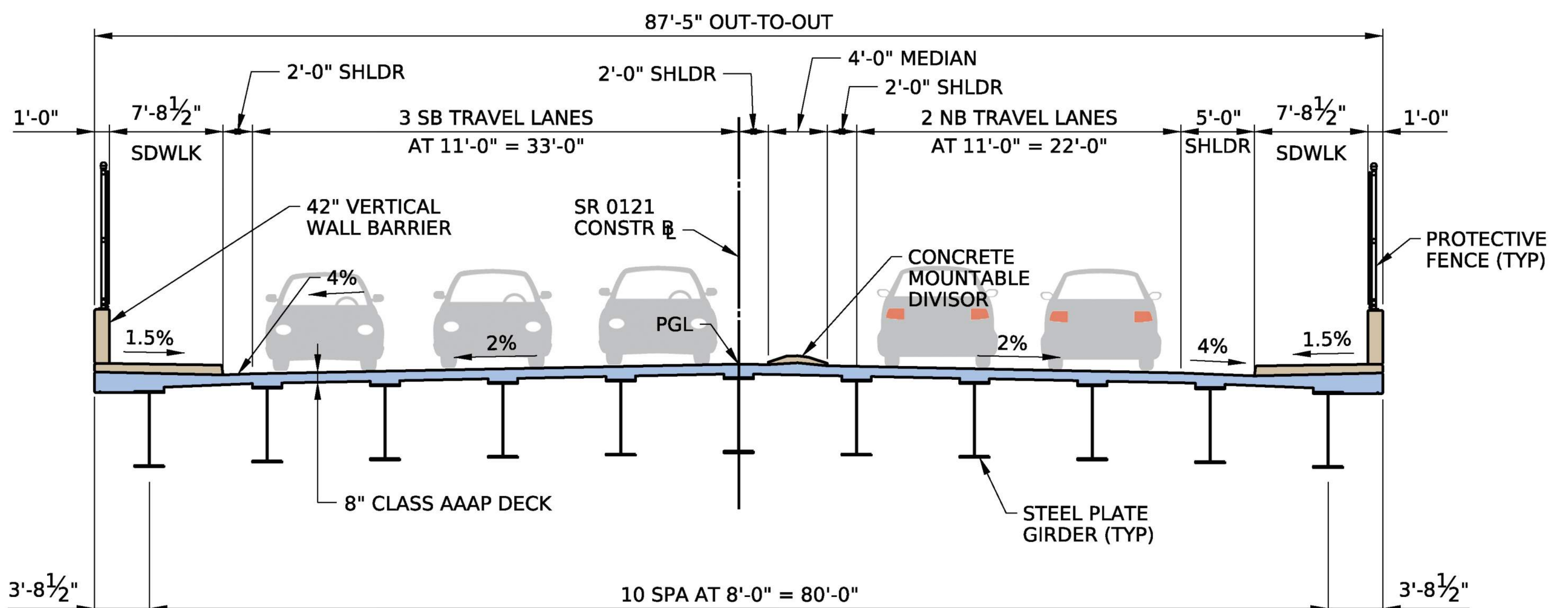
TYPICAL SECTION
