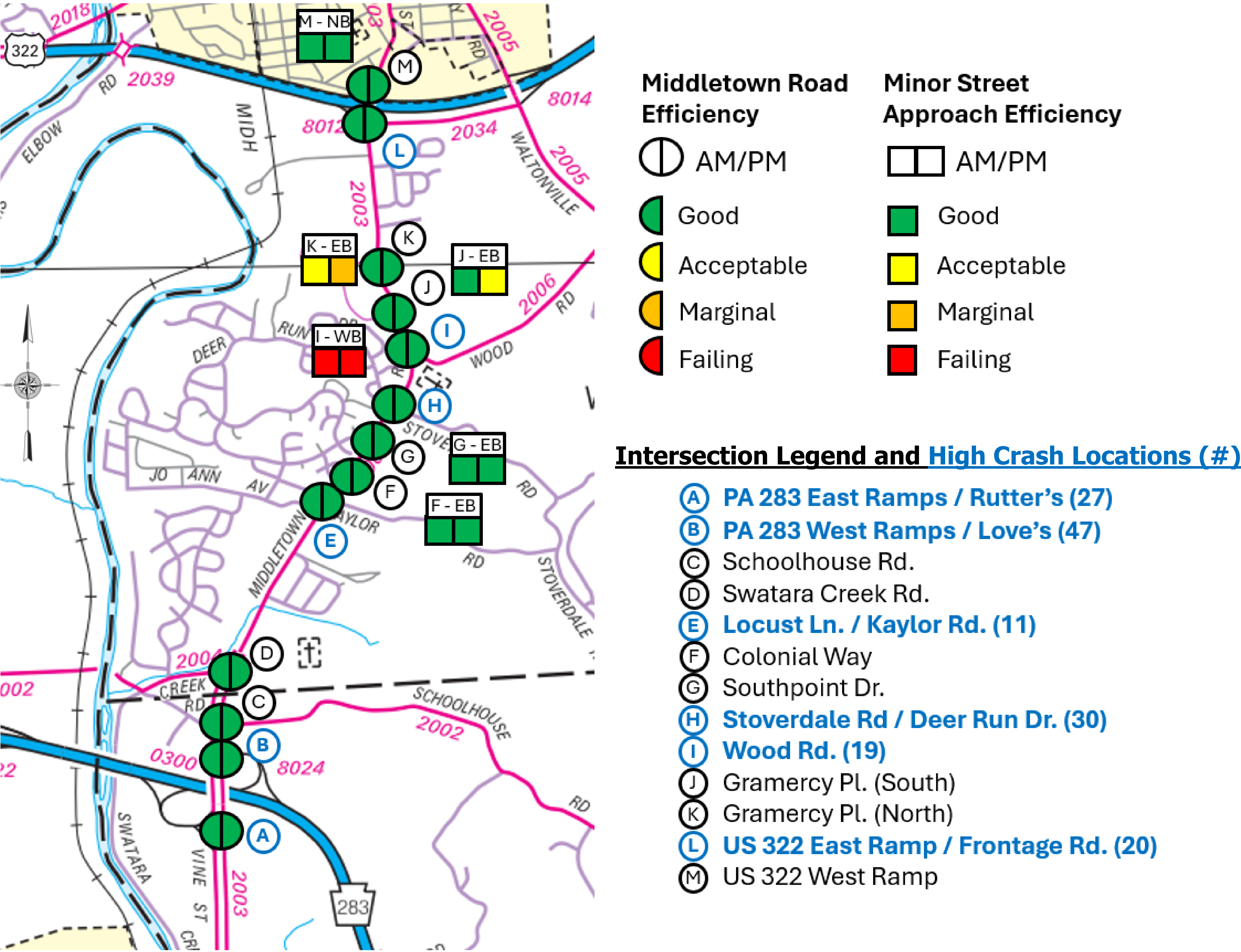
Existing Intersection Efficiency and High Crash Locations
