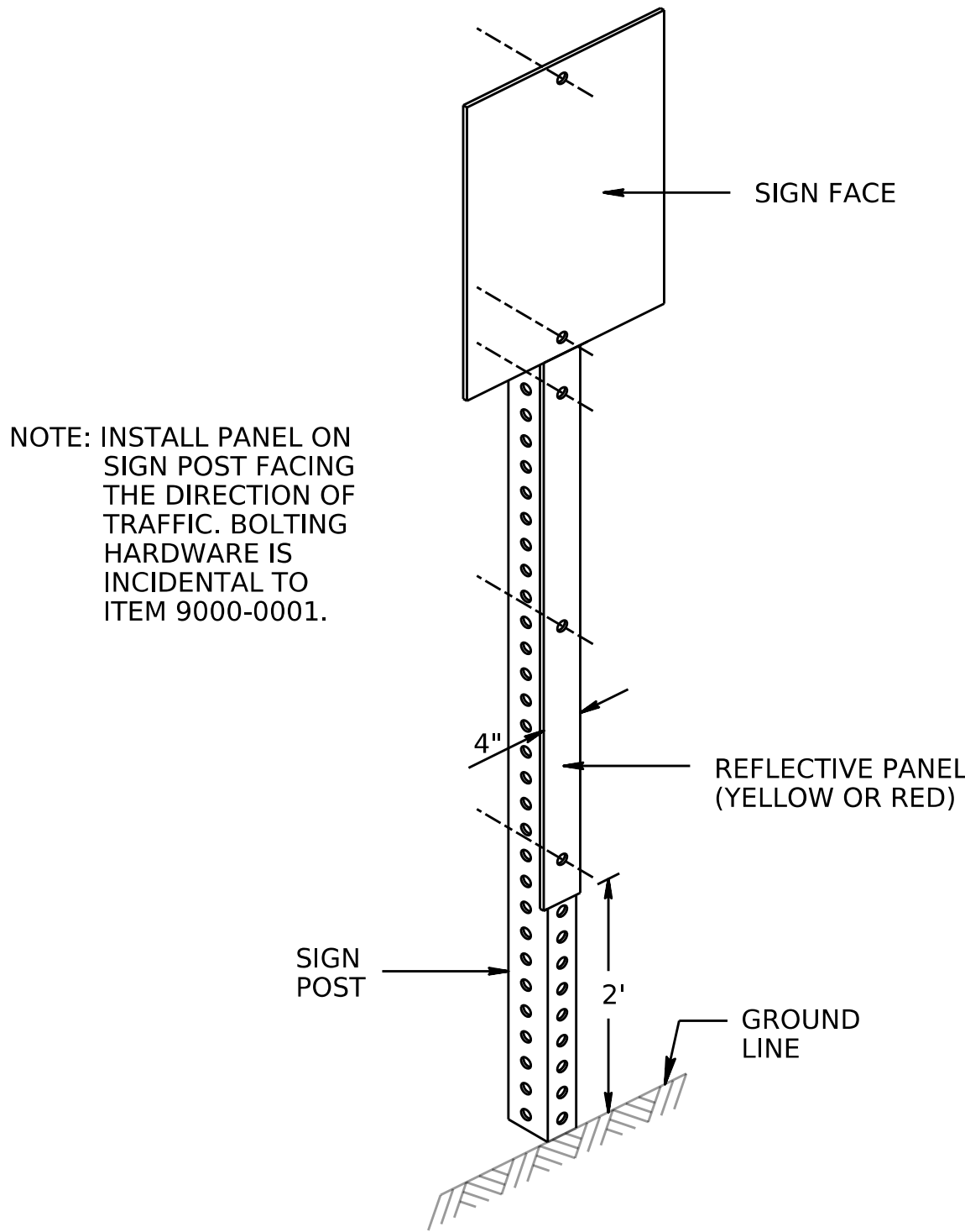
ITEM 9000-0001 - REFLECTIVE SIGN POST STRIPS DETAIL
