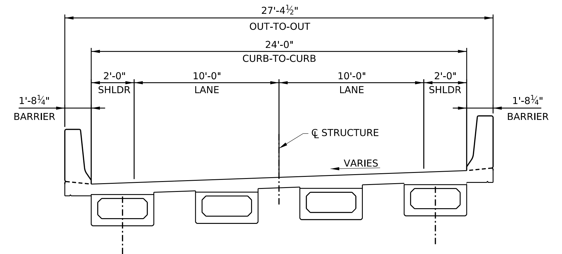
TYPICAL SECTION OF BRIDGE
