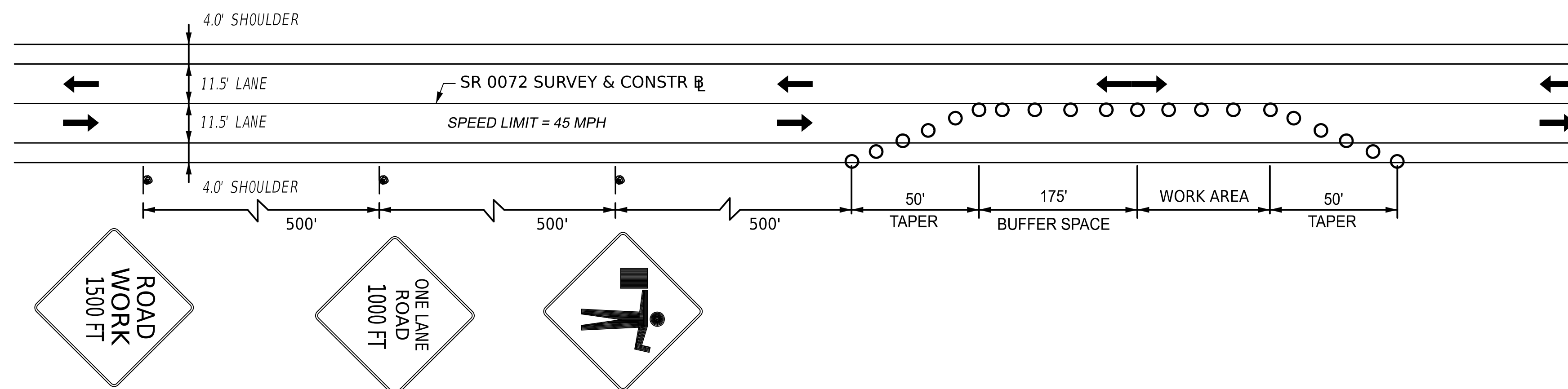
SR 0072 SHORT TERM ADVANCED WARNING SIGNS LANE CLOSED (OTHER DIRECTION SIMILAR) NOT TO SCALE
