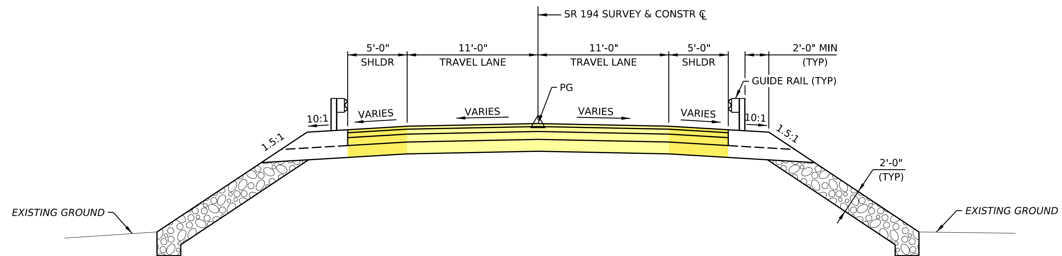
TYPICAL RECONSTRUCTION SECTION
