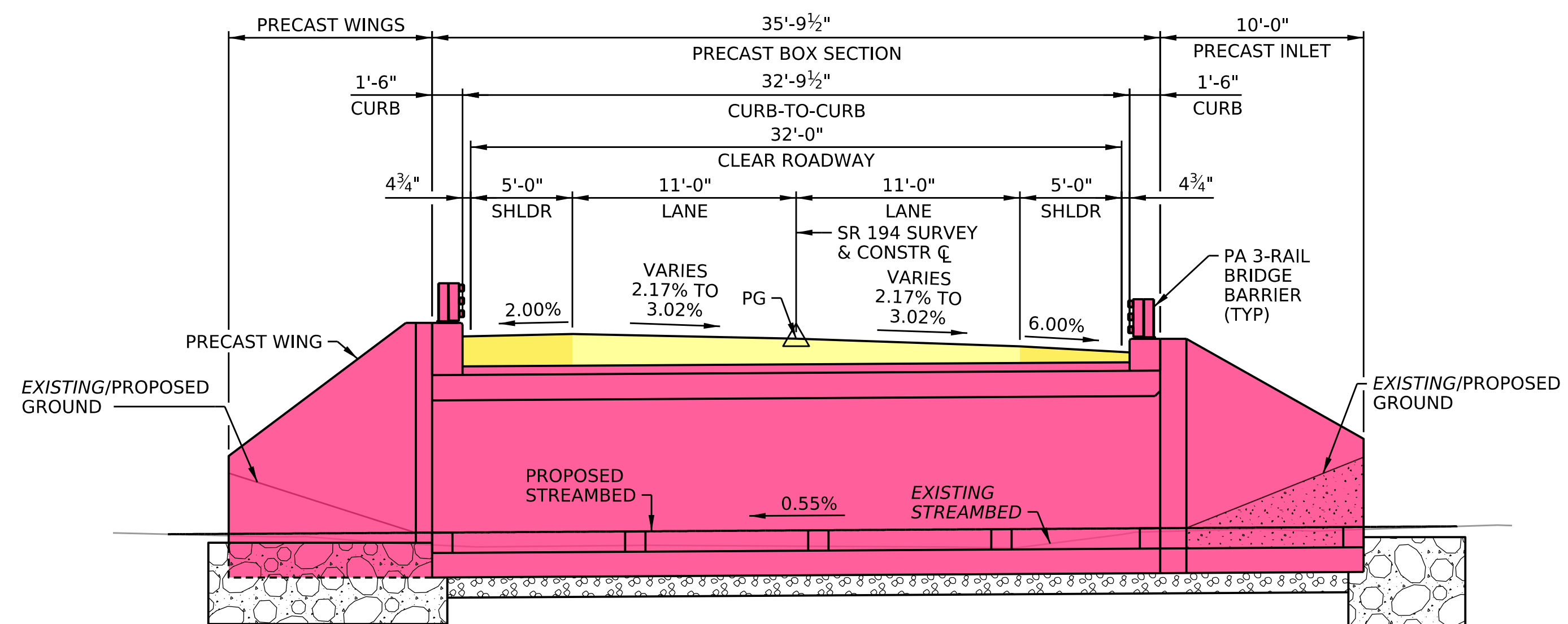
SECTION ALONG CULVERT CL
