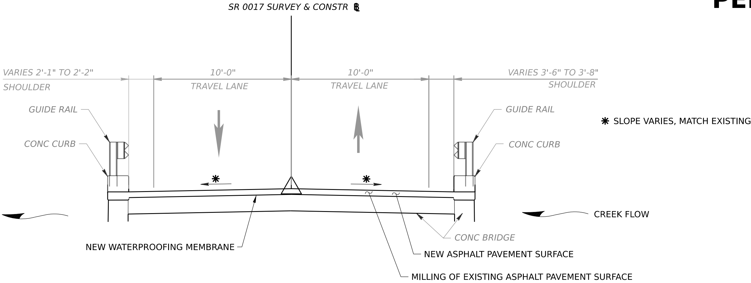
SECTION A-A BRIDGE CARRYING TRIBUTARY TO RACCOON CREEK NOT TO SCALE
