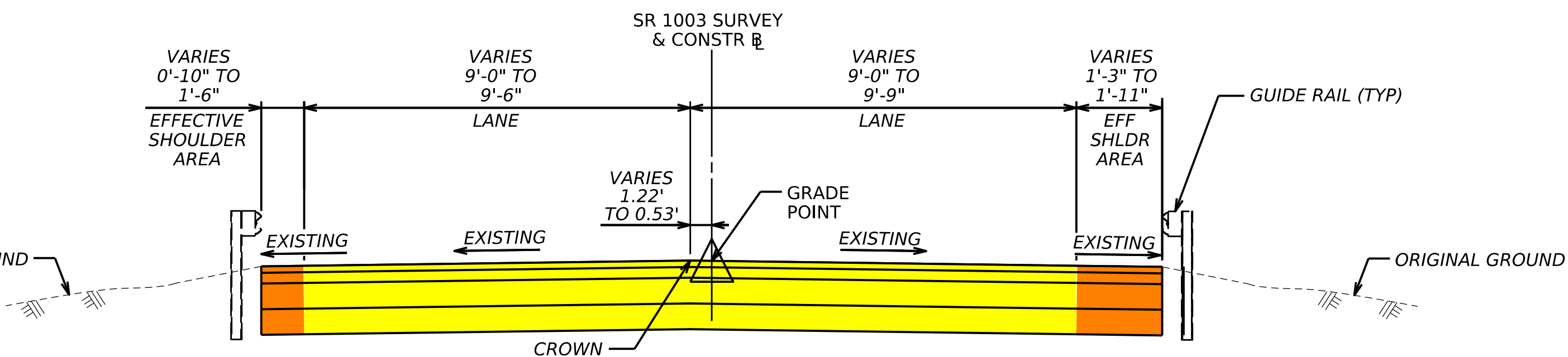
SR 1003 ROADWAY TYPICAL SECTION
