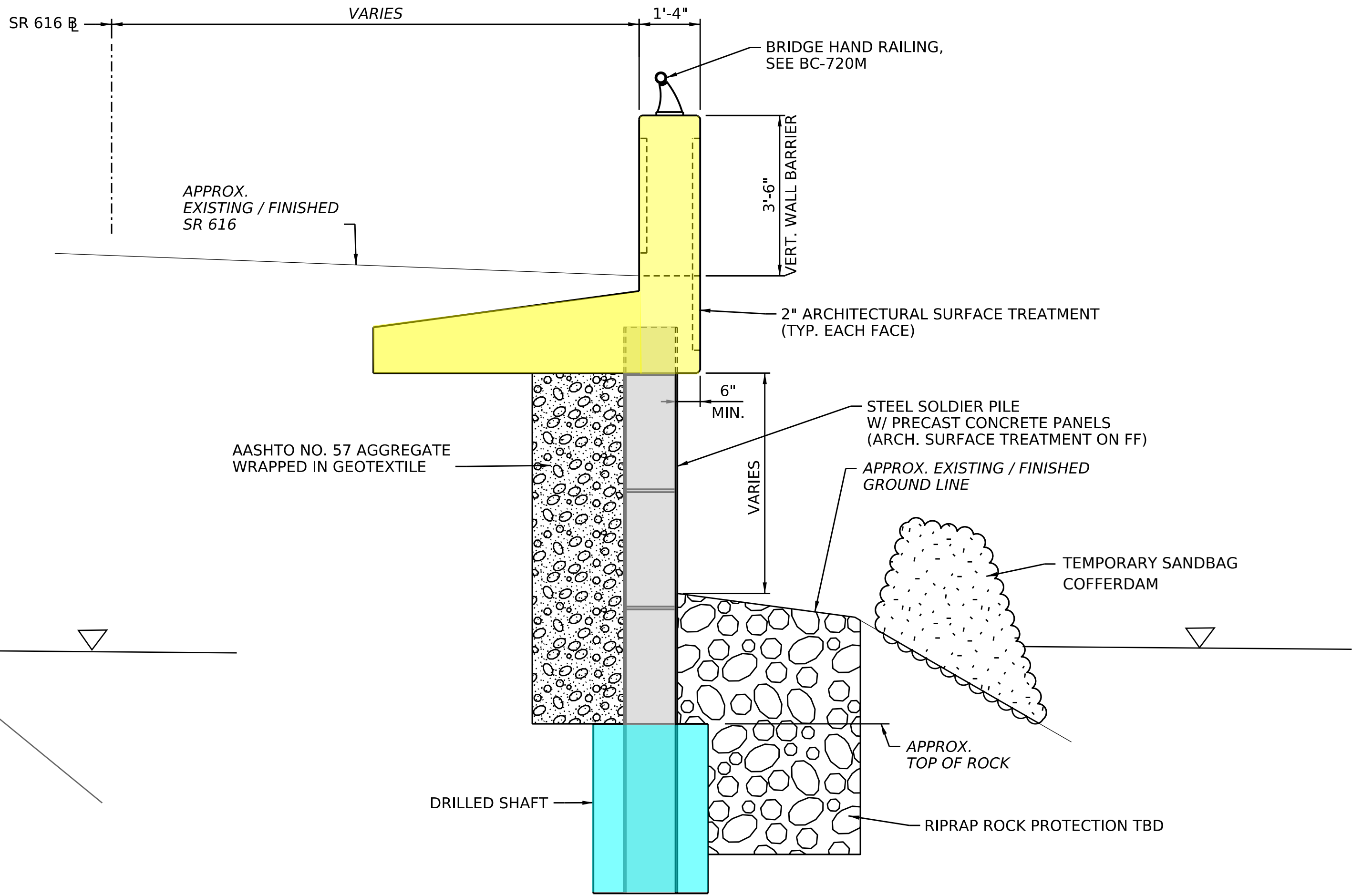
PROPOSED TYPICAL SECTION 1 0 1 2 FEET
