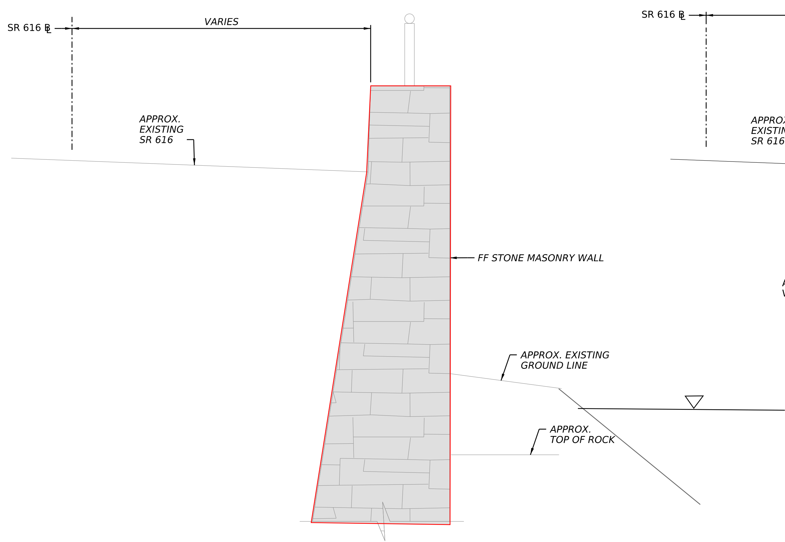
EXISTNG TYPICAL SECTION 1 0 1 2 FEET
