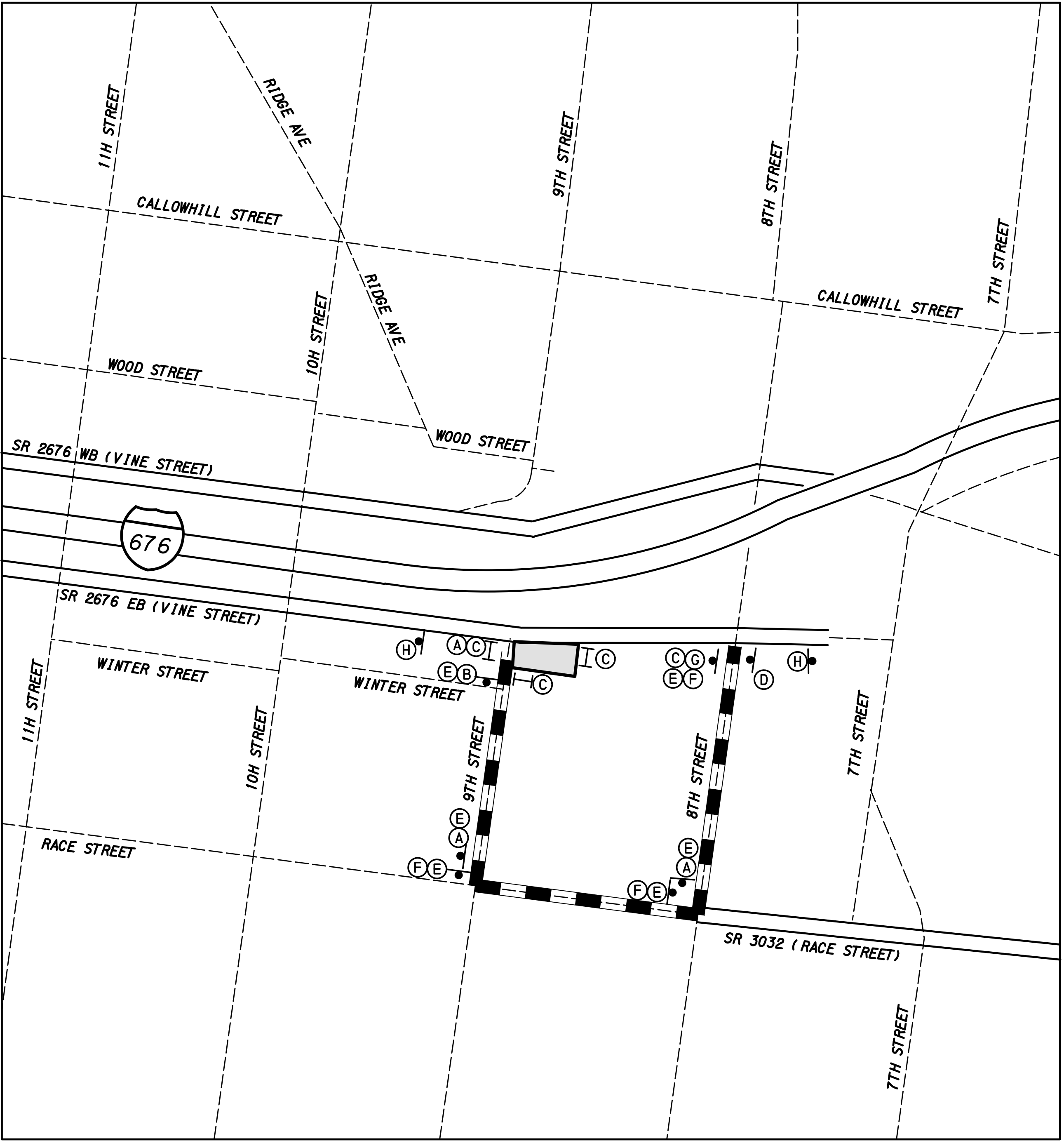
STAGE 2 PEDESTRIAN DETOUR - 9TH STREET & SR 2676 EB
