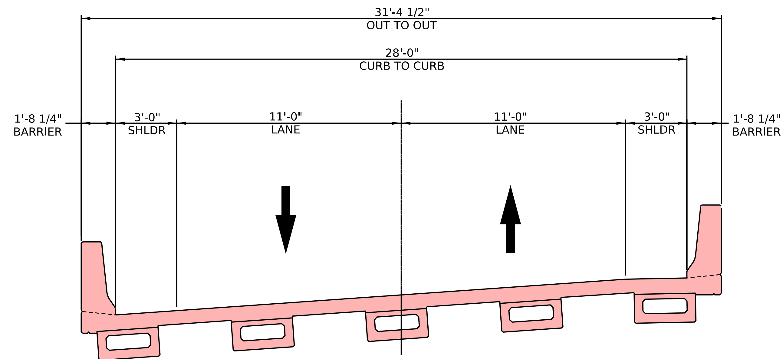
PROPOSED TYPICAL SECTION
