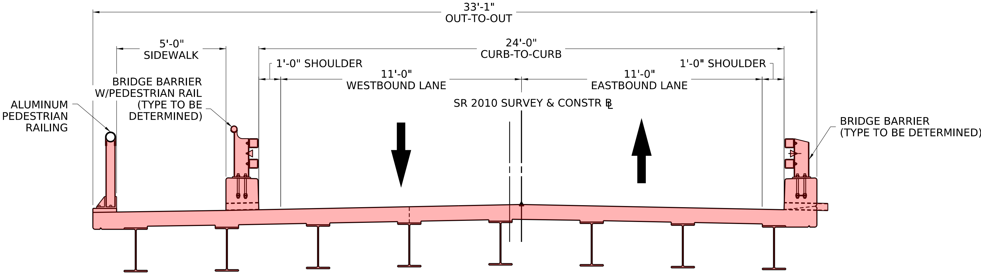
PROPOSED TYPICAL SECTION - VIEW FROM THE EAST
