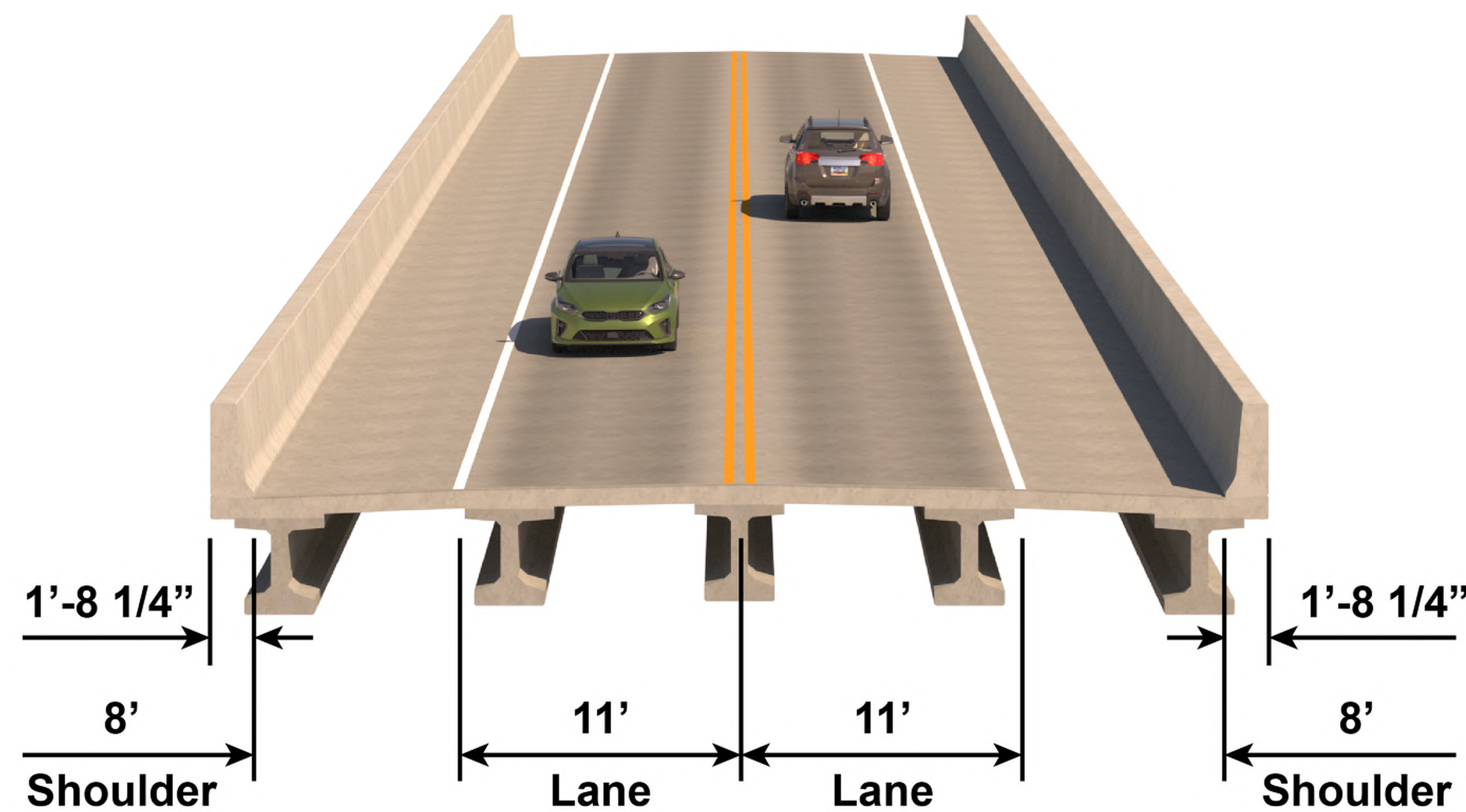
Proposed Route 4003 (Kecks Road Overpass)
