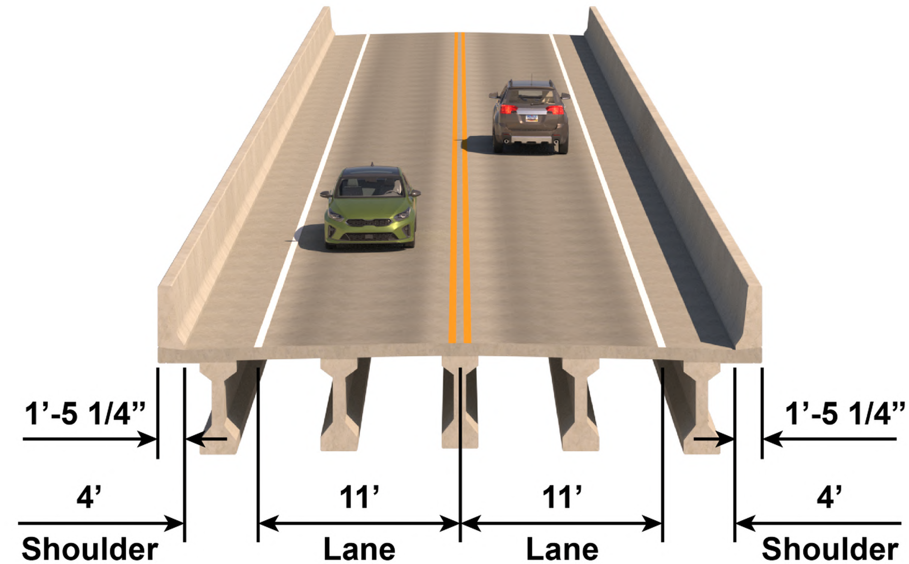
Existing Route 4003 (Kecks Road Overpass)
