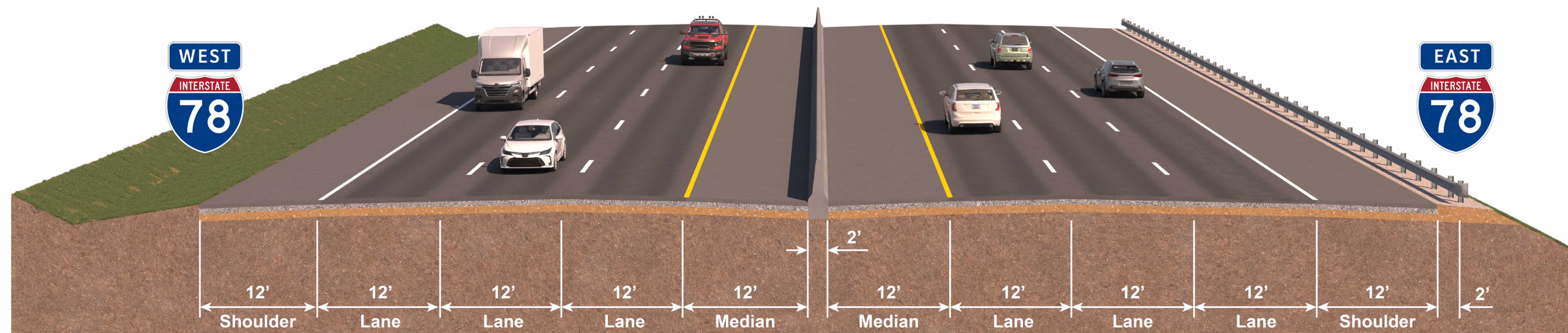
Proposed 6-Lane Configuration
