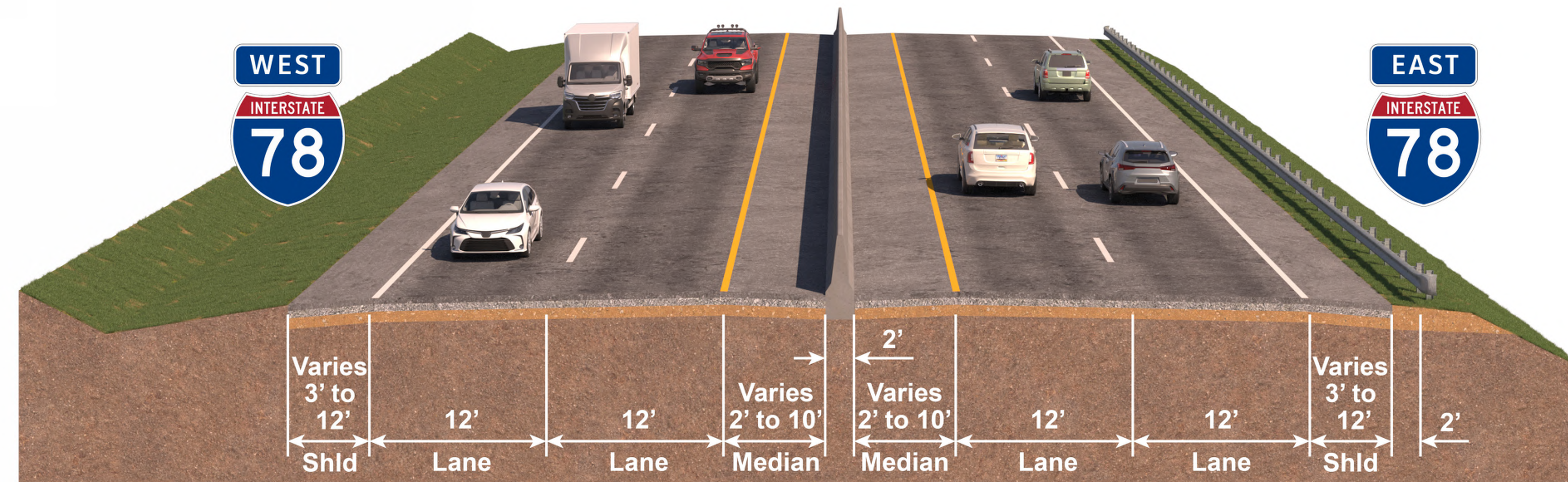
Existing 4-Lane Configuration
