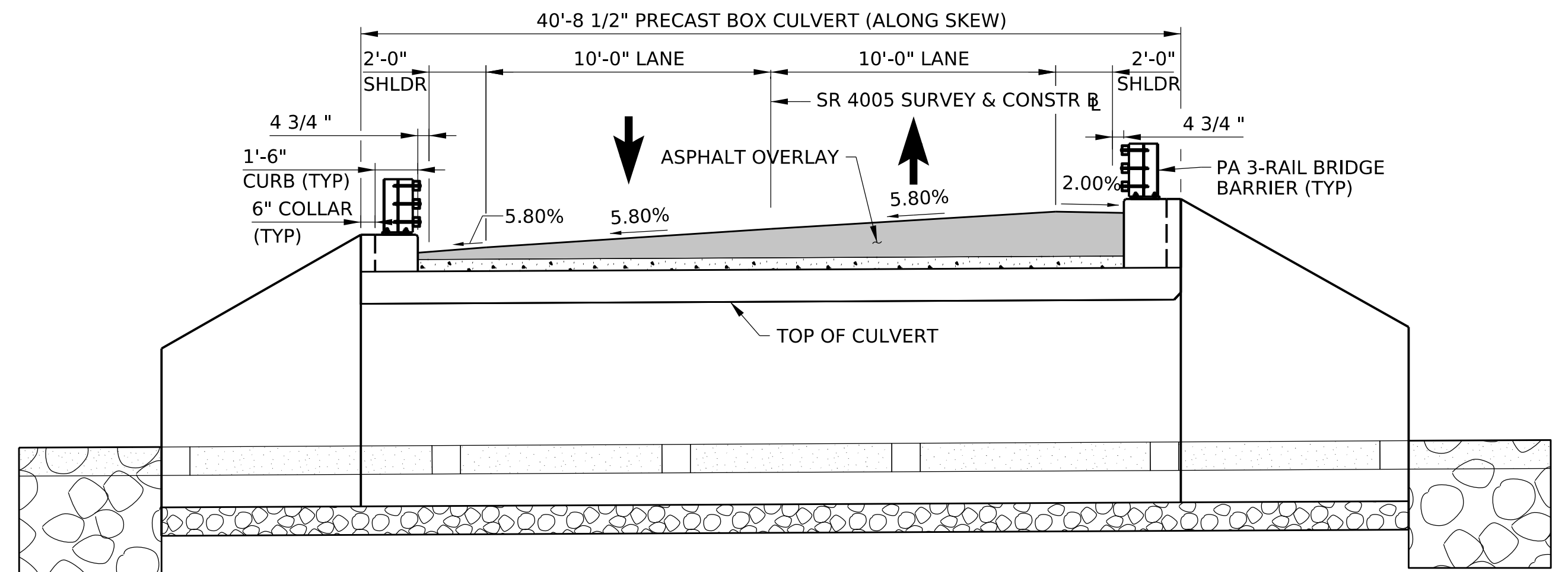
PROPOSED BRIDGE TYPICAL SECTION
