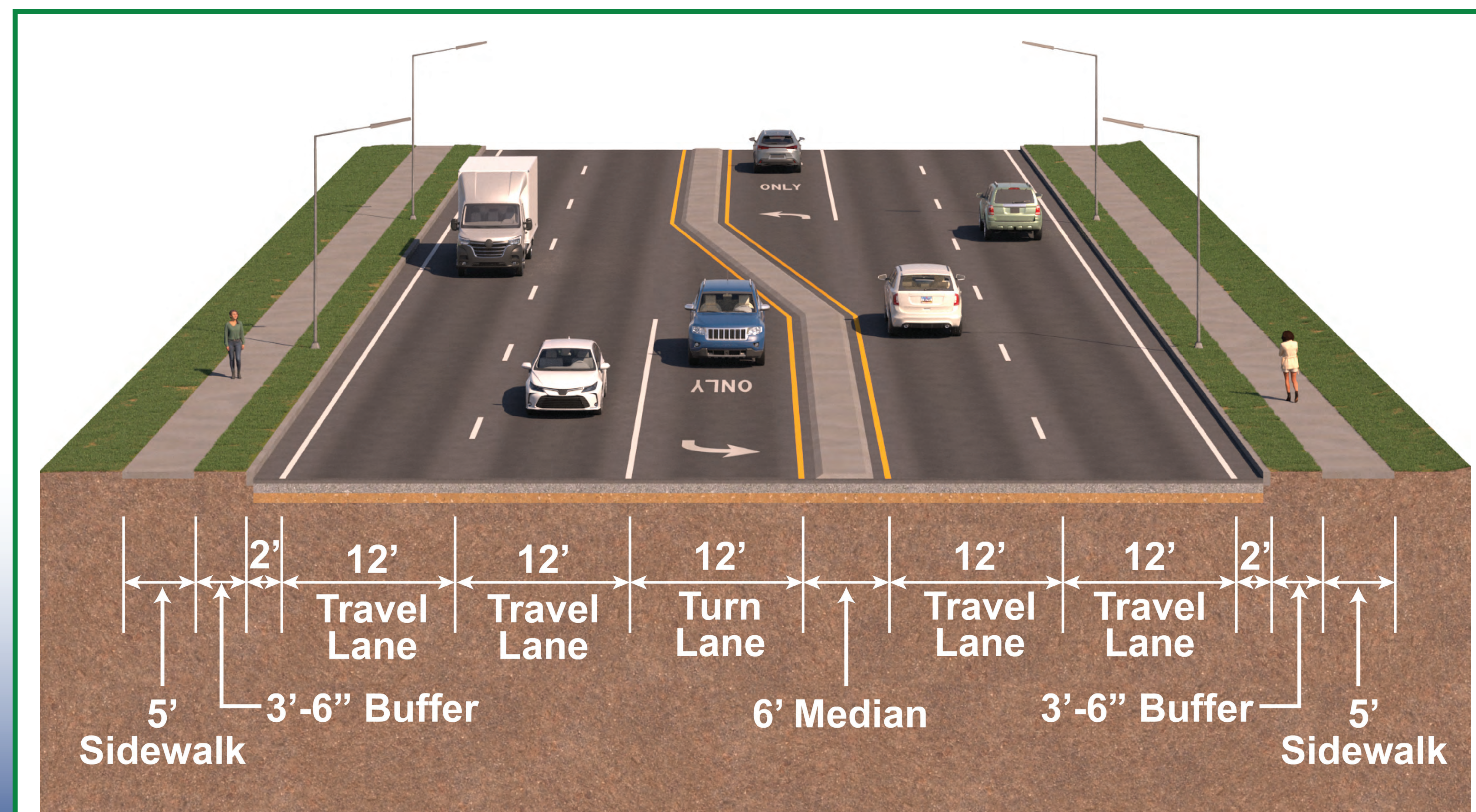
Proposed SR 191 typical section
