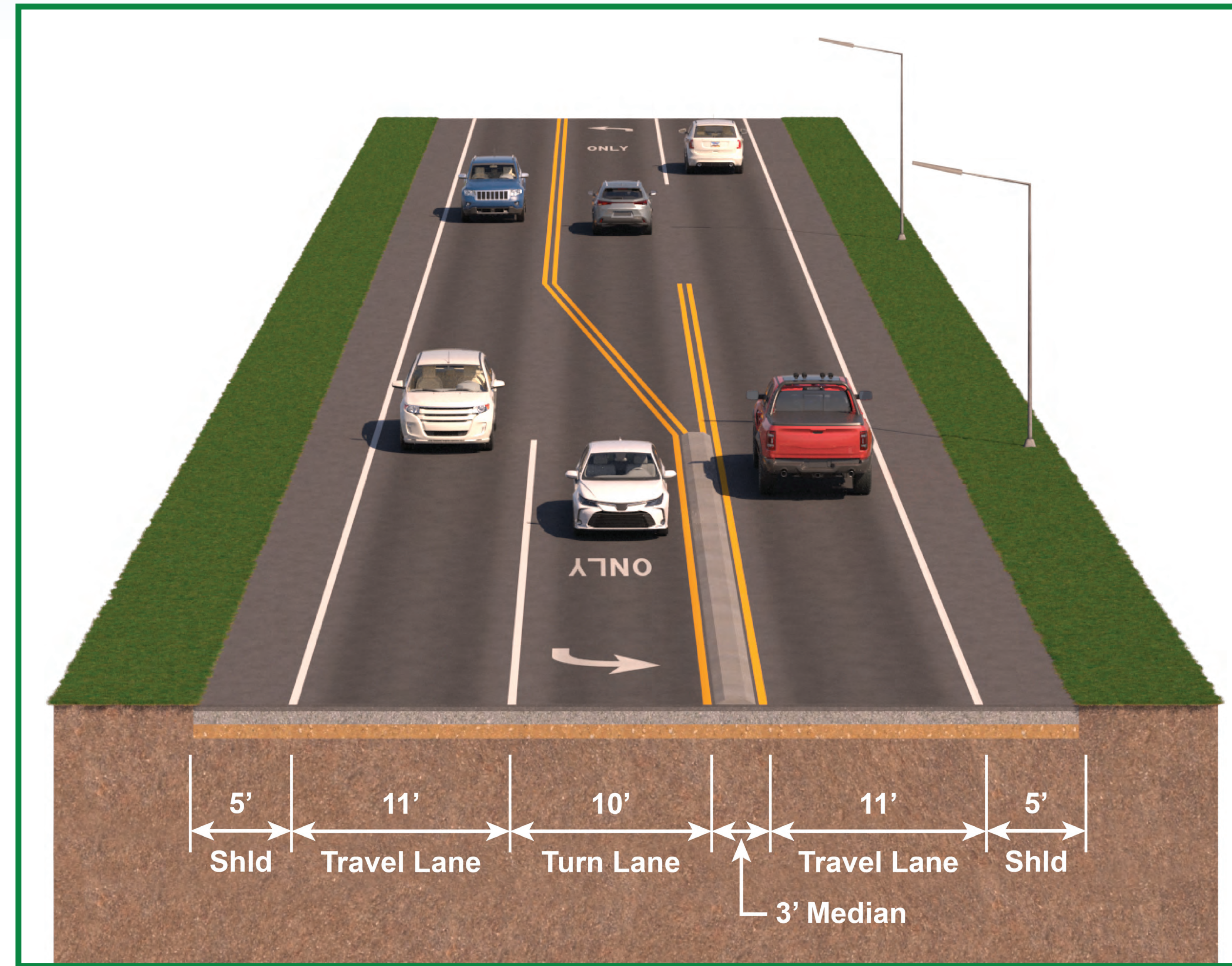
Existing SR 191 typical section
