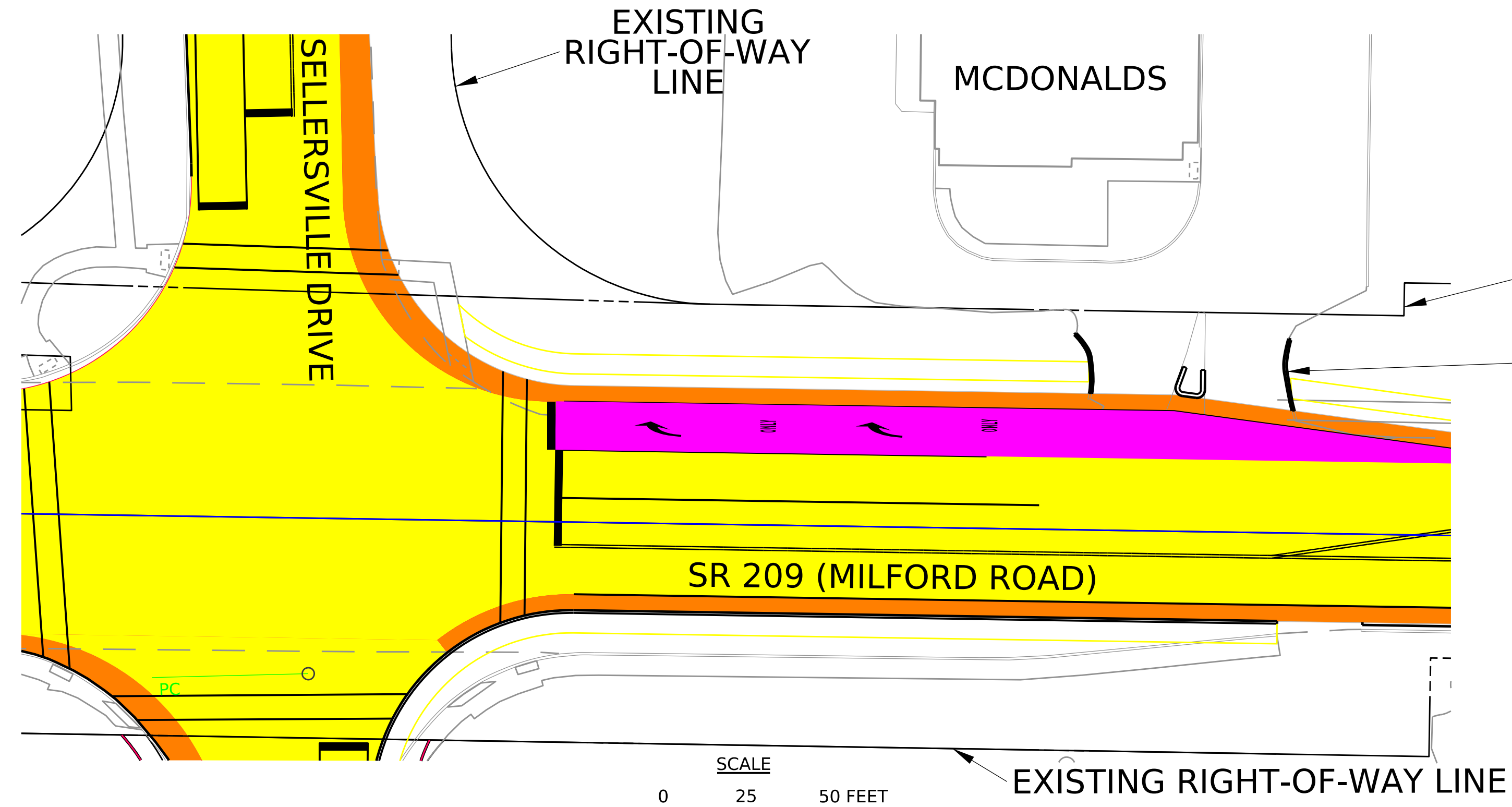
SOUTHBOUND MILFORD ROAD PROPOSED RIGHT TURN LANE AT SELLERSVILLE DRIVE
