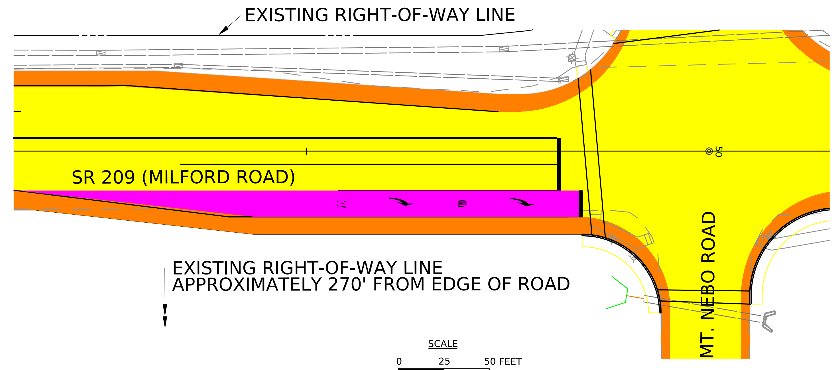
NORTHBOUND MILFORD ROAD PROPOSED RIGHT TURN LANE AT MT. NEBO ROAD
