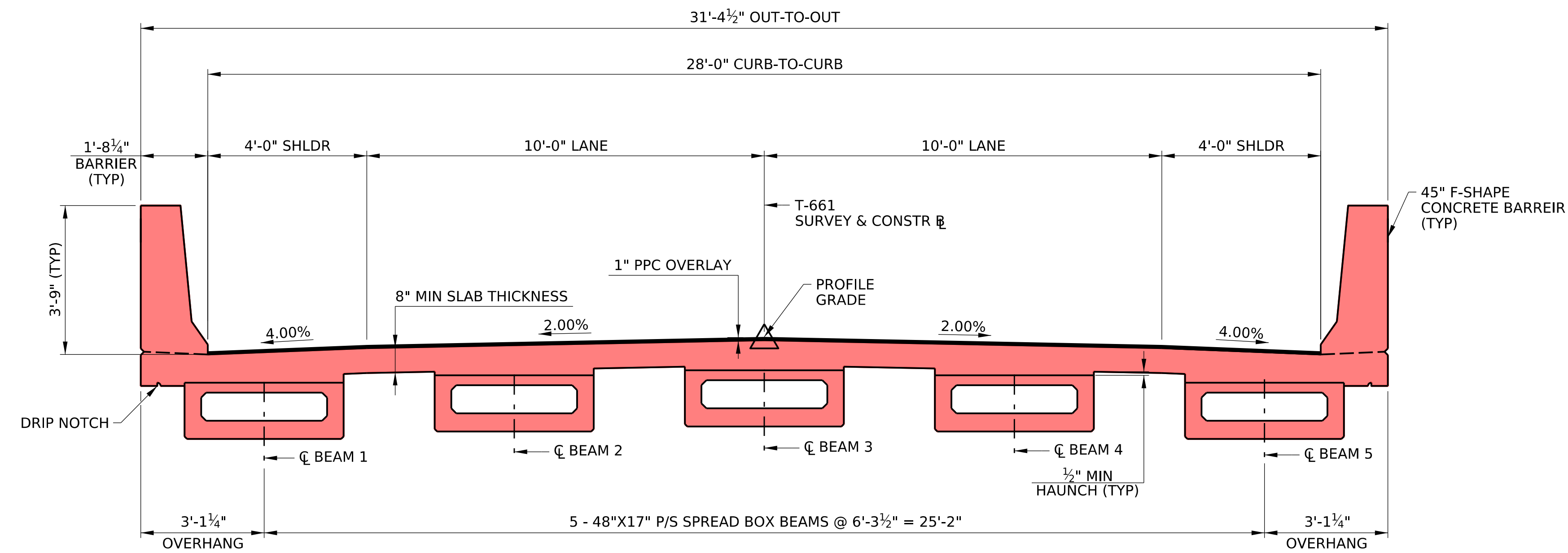
TYPICAL BRIDGE SECTION STA 10+71.92 TO STA 11+27.96 1 0 1 2 FEET
