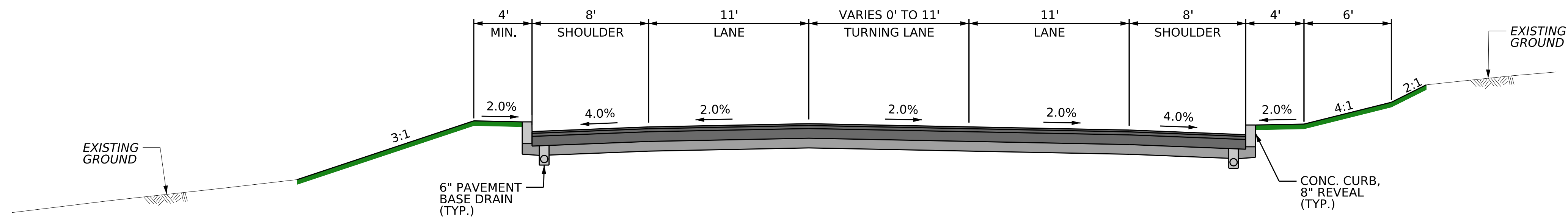
SR 0012 (PRICETOWN RD.) TYPICAL SECTION - EAST OF MT. LAUREL DR.. NOT TO SCALE
