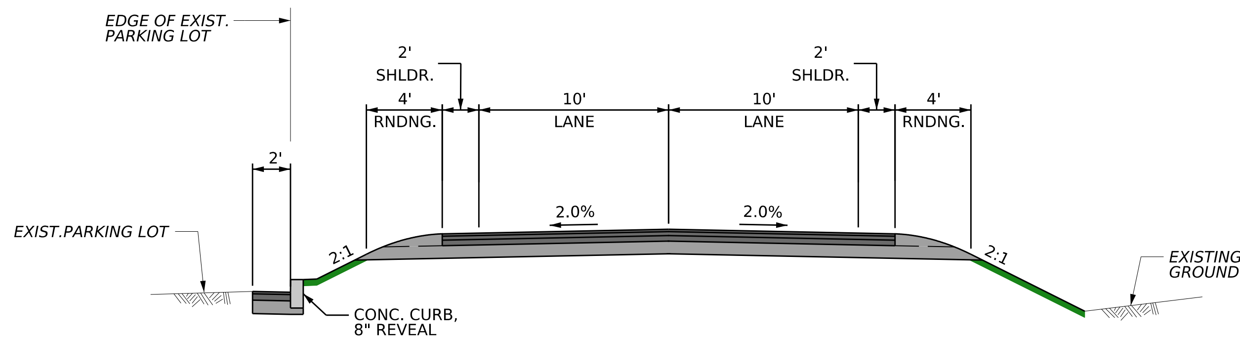
SR 1004 (MT LAUREL DR.) TYPICAL SECTION NOT TO SCALE
