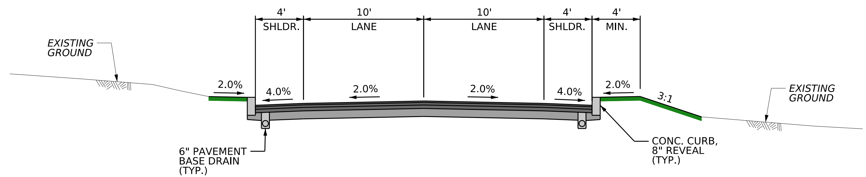
SR 2029 (ANTIETAM RD.) TYPICAL SECTION NOT TO SCALE
