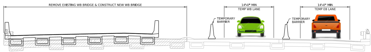
STAGE 1 TYPICAL SECTION
