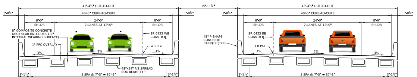
FINAL CONDITION TYPICAL SECTION
