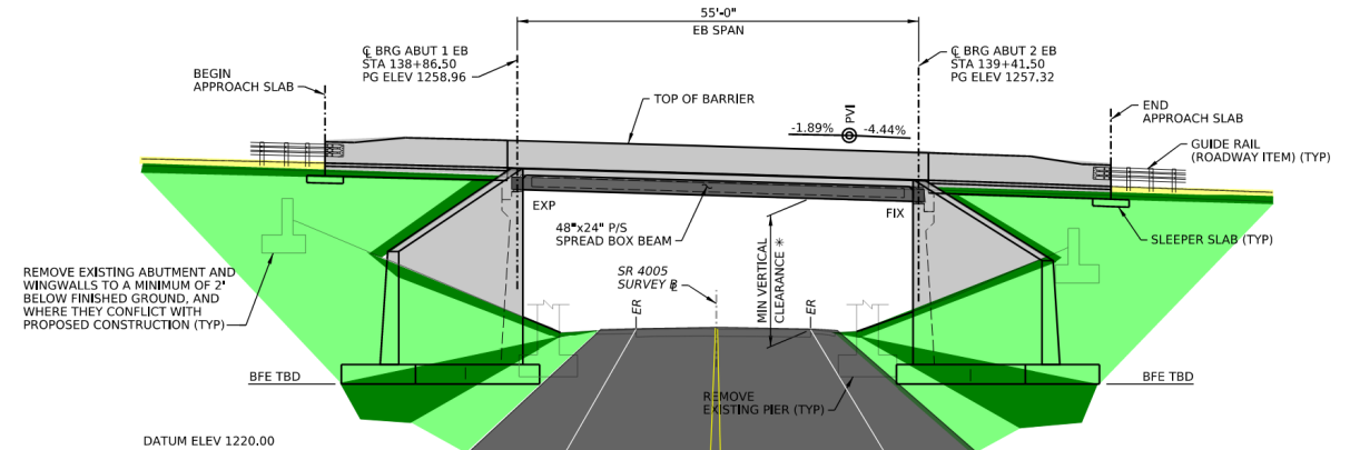
EB ELEVATION
