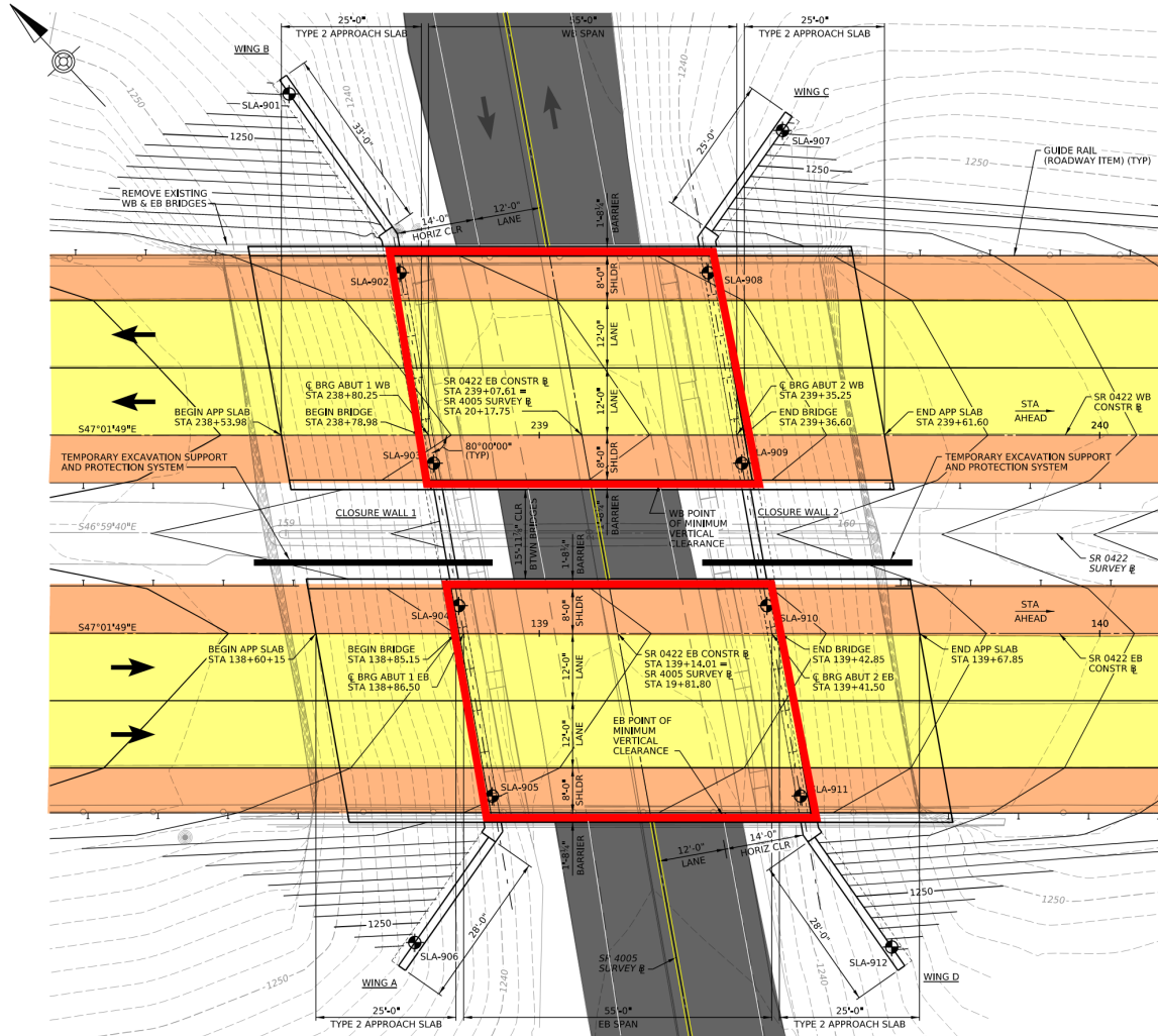
PLAN
